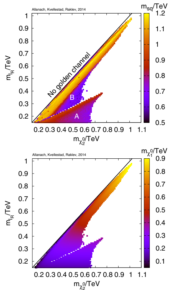
FIG. 7 (color online). Constraints on golden channel parameter space from the CMS lljj\cancel{p}_T search over the plane of pole masses of the second-lightest neutralino and the right-handed slepton. A colored box indicates a point that fits the 95% C.L. lower limit of the inferred value of CMS lljj\cancel{p}_T signal rate and is also consistent with CMS's edge inference. The squark mass (upper panel) or lightest neutralino mass (lower panel) is given by reference to the scale on the right-hand side. Above the black line, the golden channel is kinematically inaccessible.
