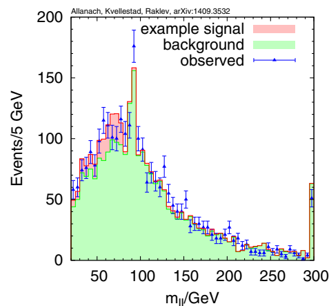
FIG. 1 (color online). Invariant mass distribution of OSSF leptons in the CMS selection after cuts. The expected Standard Model background is shown (green), which is calculated from data by using OSOF events, as well as the observed data, and an example signal point (red) in the parameter space investigated here involving the golden cascade: m_{\tilde{q}} = 900 \text{ GeV} , m_{\tilde{\chi}_2^0} = 312 \text{ GeV} , m_{\tilde{l}_R} = 200 \text{ GeV} , m_{\tilde{\chi}_1^0} = 216 \text{ GeV} . Error bars on the observed number of events show the expected statistical standard deviation.
