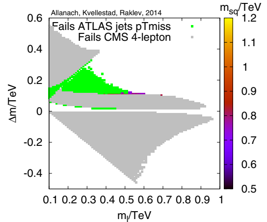
FIG. 10 (color online). Constraints on golden channel parameter space from the CMS 4l\cancel{p}_T search. The squark mass consistent with the 95% C.L. lower bound on the CMS lljj\cancel{p}_T signal is given by reference to the scale on the right-hand side. Light gray points are ruled out by the CMS 4-lepton search at the 95% C.L., whereas those colored green are ruled out by ATLAS jets \cancel{p}_T searches, at the 95% C.L.
