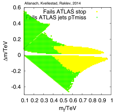
FIG. 11 (color online). Constraints on the golden channel parameter space from the ATLAS stop pair production search involving two leptons. Yellow points are ruled out by the ATLAS search for leptonically decaying stops at the 95% C.L., whereas those colored green are ruled out by ATLAS jets plus \cancel{p}_T searches at the 95% C.L.
