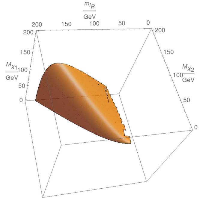
FIG. 3 (color online). Constraint on SUSY particle masses involved in the \tilde{\chi}_2^0 decay coming from the central value m_{ll}^{\max} = 78.7 GeV.
