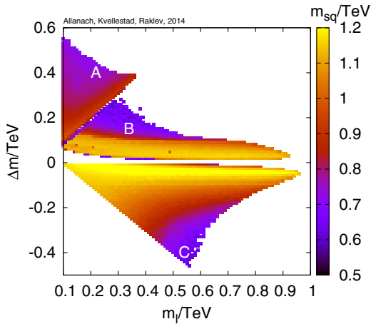
FIG. 6 (color online). Constraints on golden channel parameter space from the CMS lljj\cancel{p}_T search over the input parameter plane m_{\tilde{1}}(M_{\text{SUSY}}) and \Delta m = M_2(M_{\text{SUSY}}) - m_{\tilde{1}}(M_{\text{SUSY}}) . A colored box indicates a point that fits the 95% C.L. lower limit of the inferred value of CMS lljj\cancel{p}_T signal rate and is also consistent with CMS's edge inference.
