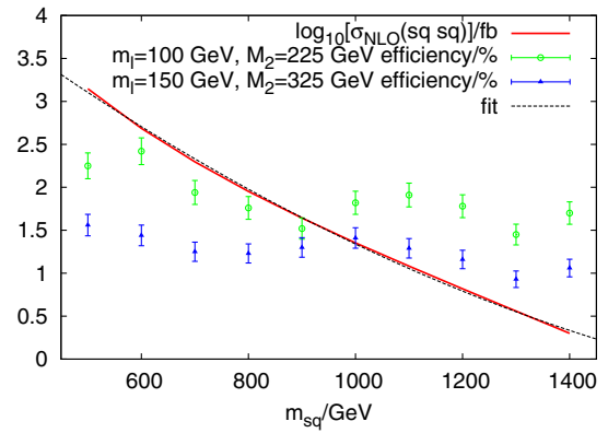
FIG. 5 (color online). Fit to (anti)squark production cross section at an 8 TeV LHC. The logarithm of the PROSPINO cross section prediction is shown by the solid line. Our quadratic fit to this is shown by the dashed line. The CMS lljj\cancel{p}_T search region cut efficiencies for two parameter space points are shown by the points with errorbars, where the errorbars are purely from Monte Carlo statistics.
