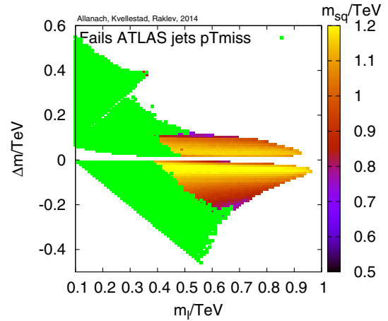
FIG. 8 (color online). Constraints on golden channel parameter space from the ATLAS jets plus \cancel{p}_T search. The squark mass consistent with the 95% C.L. lower bound on the CMS lljj\cancel{p}_T signal is given by reference to the scale on the right-hand side. Points colored green are excluded by an ATLAS \cancel{p}_T plus jets search at the 95% C.L.
