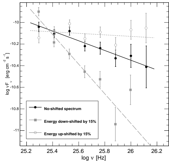
Figure 4. MAGIC spectral energy distribution EBL-corrected with Franceschini et al. (2008) model by assuming z = 0.4 . The no-shifted spectrum is represented by the black circles. The solid grey squares show the spectrum considering a shift to lower energies by 15%, and the grey open circles represent the spectrum accounting for a shift to higher energies by 15%.
