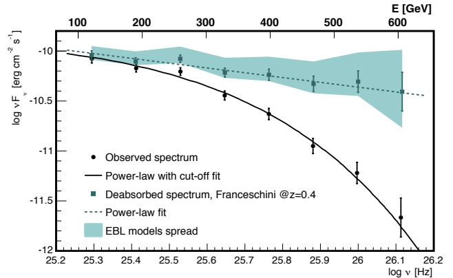
Figure 3. SED of PG 1553+113 as measured by MAGIC during the flare state of 2012 April. The observed SED is shown as black circles, and the black solid line represents the best fit to a power law with an exponential cut-off. The absorption-corrected spectrum assuming z = 0.4 and using the EBL model by Franceschini et al. (2008) is shown by the green squares; the dashed green line is the best-fitting power law. The green shaded area accounts for the uncertainties derived by the use of different EBL models.
