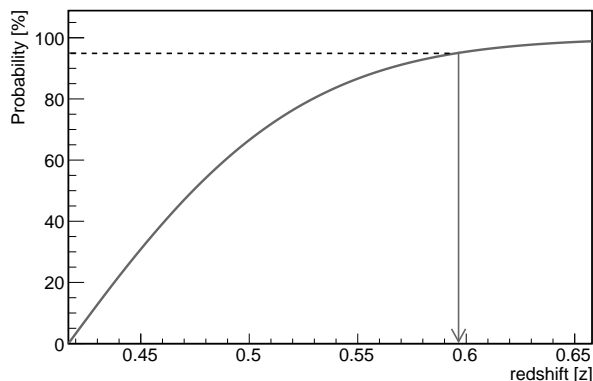
Figure 5. Constraint on the redshift of PG 1553+113 with the likelihood ratio test when comparing the hypothesis of a power-law fit and a positive curved power law (concave upward) fit for different distances of the source, using the EBL model from Franceschini et al. (2008).
