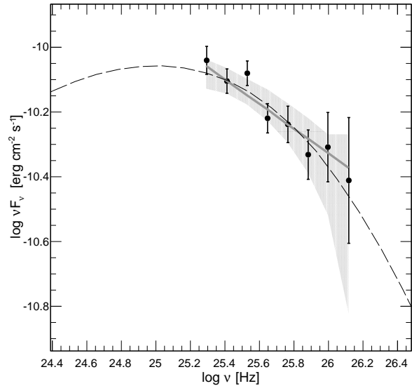
Figure 7. PG 1553+113 VHE SED. The gray shaded area represents the simulated MAGIC response assuming the intrinsic emission given by the best-fitting SSC model to the MWL data shown in Fig. 6. The gray solid line represents the mean power-law fit of the ten thousand realizations of the toy-MC. The black circles denote the PG 1553+113 VHE spectrum EBL-corrected with Franceschini et al. (2008) model assuming z=0.4 . The dashed black line represent the best-fitting SSC model from Fig. 6.
