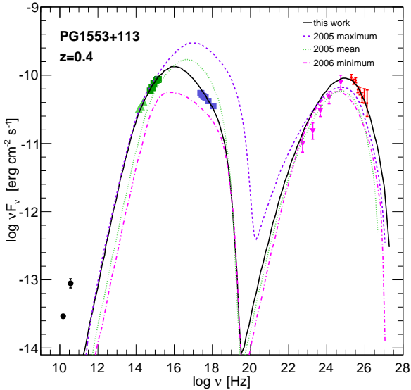
Figure 6. Spectral energy distribution of PG 1553+113 during the 2012 April flare state modeled with the one-zone SSC model of Maraschi & Tavecchio (1993). From high to low energies: the EBL-corrected MAGIC spectra using Franceschini et al. (2008) assuming z=0.4 (red dots, see text), the Fermi -LAT data from MJD 55959-56088 (pink triangles), Swift -XRT (purple squares) and Swift -UVOT (green squares) data from MJD 56045 (good representation of the X-ray and optical-UV state during the VHE flare), IR data from REM (green triangles) from MJD 56047, Metsähovi (black square) from MJD 55994 (single detection) and mean radio observation in the period MJD 55959-56088 from OVRO (black circle). For comparison, the SSC models for previous source states (Aleksić et al. 2012a) have been plotted in colored dashed lines.
