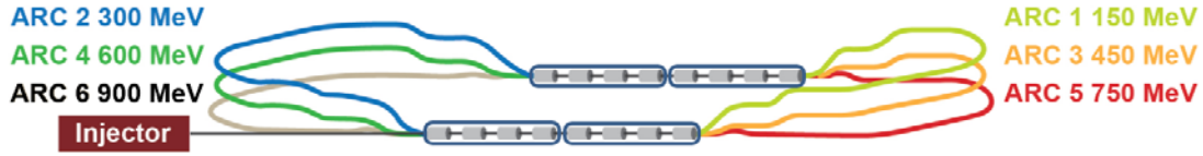
Figure 1: Conceptual layout of the ERL Test Facility
