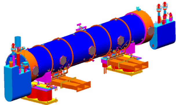
Figure 3: Conceptual design of the 802 MHz CM, SNS style [6]
