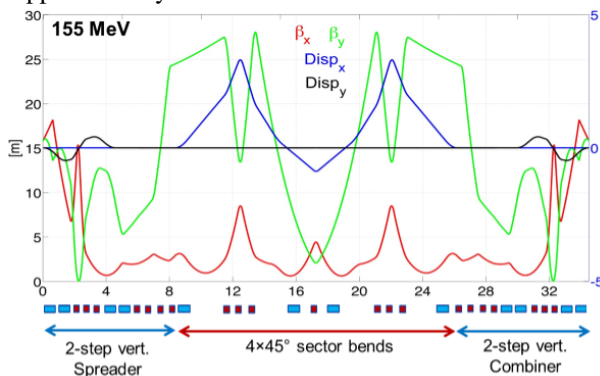
Figure 4: Optics based on an FMC cell of the lowest energy return arc at 155 MeV. Horizontal (red curve) and vertical (green curve) \beta -functions are shown. Blue and black curves show horizontal and vertical dispersion, respectively.
