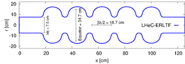
Figure 2: Approximate dimensions of a 5-cell cavity for 802 MHz
