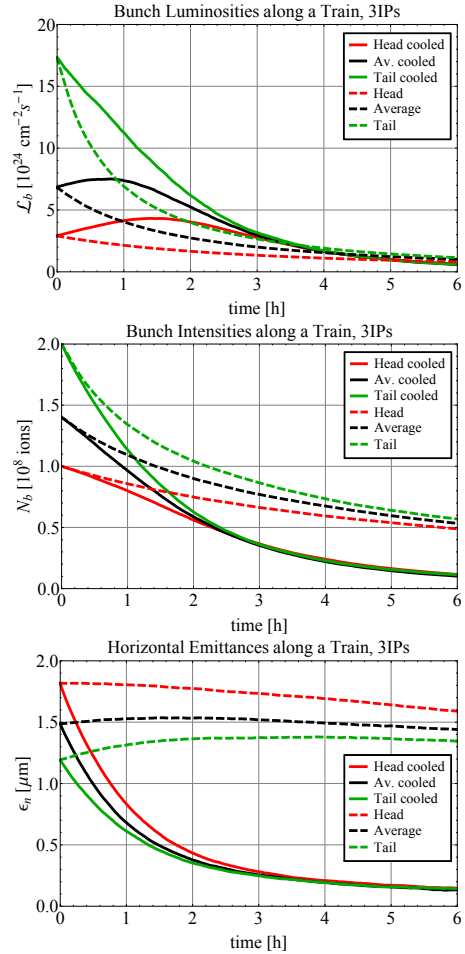
Figure 1: Beam and luminosity evolution with and without cooling for the three bunches from Table 1.
