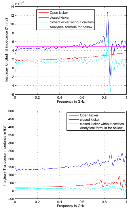
Figure 2: Longitudinal and transverse simulated impedances of RHIC kicker open (red), closed (blue), closed with cavities filled by metal (cyan) and the formula in [9] (magenta).
