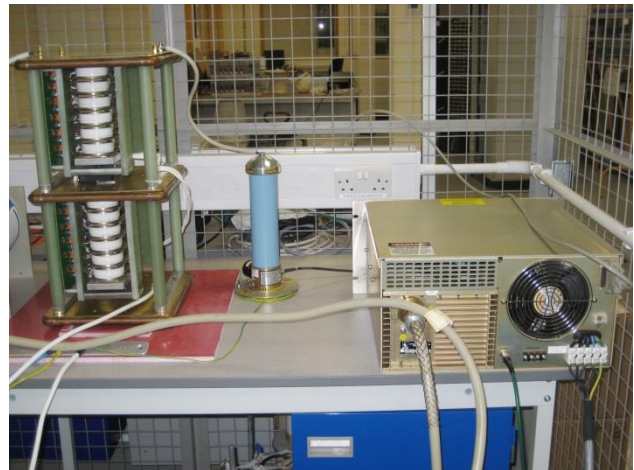
Figure 4: solid state crowbar under test at 38kV
