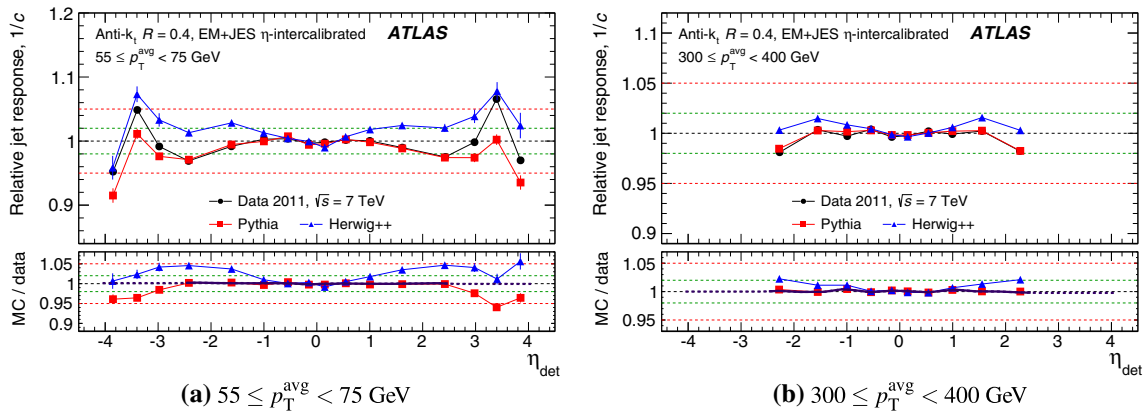
Fig. 34 Relative jet response, 1/c , as a function of the jet \eta_{\text{det}} for anti- k_r jets with R = 0.4 calibrated with the EM+JES scheme and in addition the derived \eta -intercalibration. Results are shown separately for a 55 \leq p_T^{\text{avg}} < 75 GeV and b 300 \leq p_T^{\text{avg}} < 400 GeV. For all points included in the original calibration ( |\eta_{\text{det}}| < 2.8 ), the data are corrected
