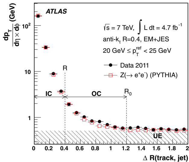
Fig. 18 Transverse momentum profile of tracks around the leading jet axis for events with 20 \leq p_T^{\text{ref}} < 25 \text{ GeV} in Z-jet events. The radii R and R_0 are those used in Eq. (12) to define the IC and IC+OC regions. The hatched area indicates the contribution from the underlying event (UE). Anti- k_t jets with R = 0.4 calibrated with the EM+JES scheme are considered
