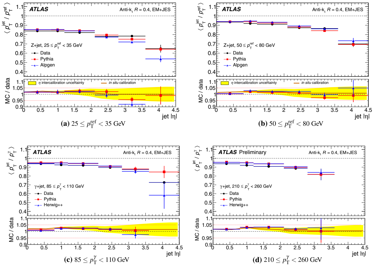
Fig. 35 The (a, b) Z-jet and (a, b) \gamma -jet balance for anti- k_r jets with R = 0.4 , calibrated with the EM+JES scheme. In a and b the results for events with 25 \leq p_T^{\text{ref}} < 35 GeV and 50 \leq p_T^{\text{ref}} < 80 GeV are shown, respectively. Here p_T^{\text{ref}} is the p_T of the reconstructed Z boson projected onto the axis of the balancing jet. The p_T balance for \gamma -jet events with photons with transverse momenta p_T^\gamma within 85 \leq p_T^\gamma < 110 GeV is shown in c , while d shows the p_T balance for higher photon transverse
