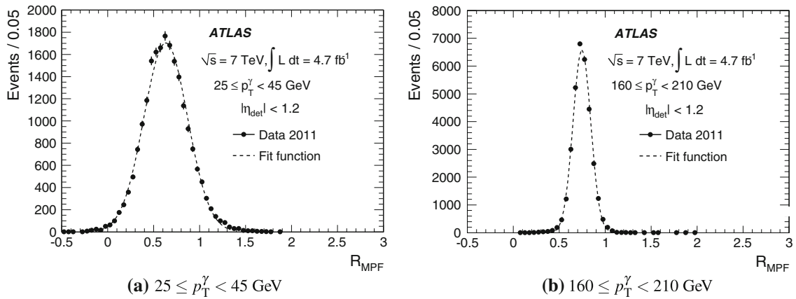
Fig. 21 MPF response distributions in the \gamma -jet data for a 25 \leq p_T^\gamma < 45 GeV and b 160 \leq p_T^\gamma < 210 GeV when using topo-clusters at the EM scale. The dashed lines represent the fits with a Gaussian function.
