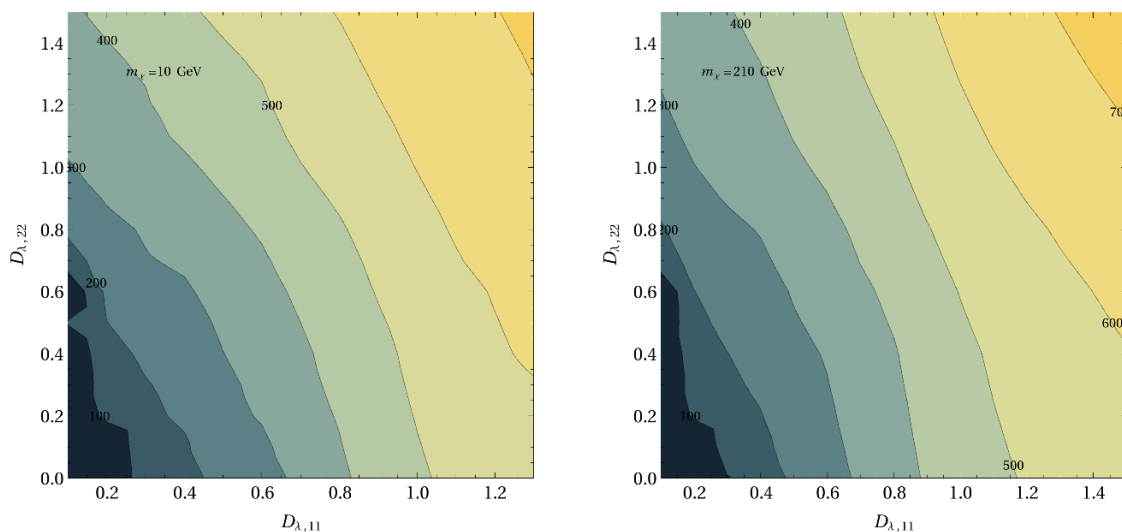
Figure 17. Limits on the mDMFV model in terms of mass of \phi (in GeV) from the CMS monojet search [71]. Limits are obtained by matching production cross sections in our model with those in the DMEFT used by CMS.
