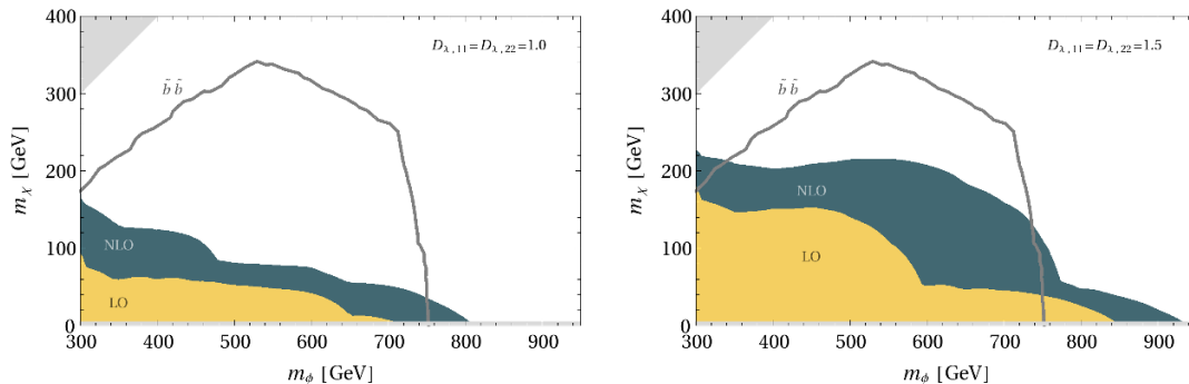
Figure 15. Limits on the mDMFV model from the CMS 19.5 \text{ fb}^{-1} sbottom [66] and squark [67] search. We show for comparison the CMS \tilde{b}\tilde{b} limit (grey curve), which also directly applies to the case D_{\lambda,11} = D_{\lambda,22} = 0 . Shaded regions are excluded for particular choices of D_{\lambda,11} and D_{\lambda,22} as shown on the plot. For the NLO limit, we estimate the cross section by multiplying LO prediction with the NLO K-factor from sbottom pair production. The DM coupling to b -quark, D_{\lambda,33} is fixed everywhere by the corresponding relic abundance constraint, and all mixing angles are set to zero for simplicity.
