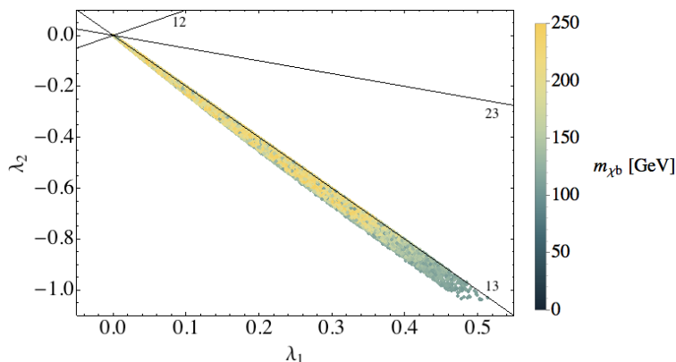
Figure 12. Allowed region in the \lambda_1 - \lambda_2 -plane for the 13-degeneracy scenario, after imposing the relic abundance, LUX and flavor constraints. The DM mass m_{\chi_b} is indicated by the color, and the ij -degeneracy lines are sketched.
