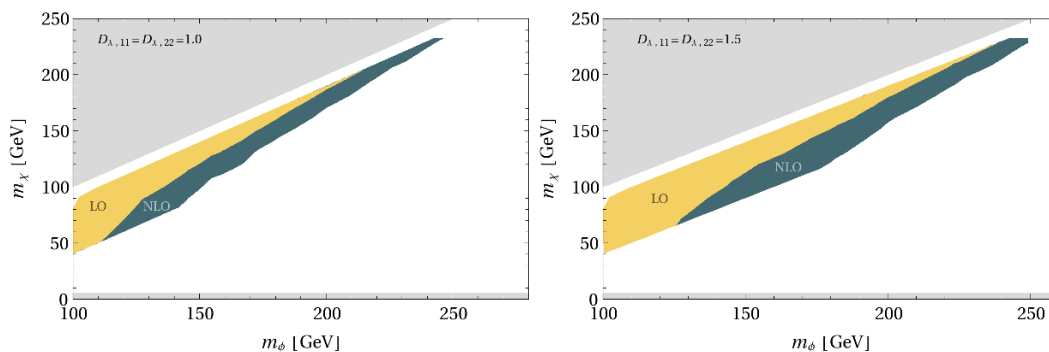
Figure 18. Limits on the mDMFV model from the CMS 19.7 \text{ fb}^{-1} search [72] for stops decaying to a charm and a neutralino, using the monojet + MET final state. The NLO cross section is estimated from the LO prediction with the NLO K-factor from sbottom pair production. The triangular grey regions are parts of parameter space where \phi is lighter than the dark matter particles and hence cannot decay into them.
