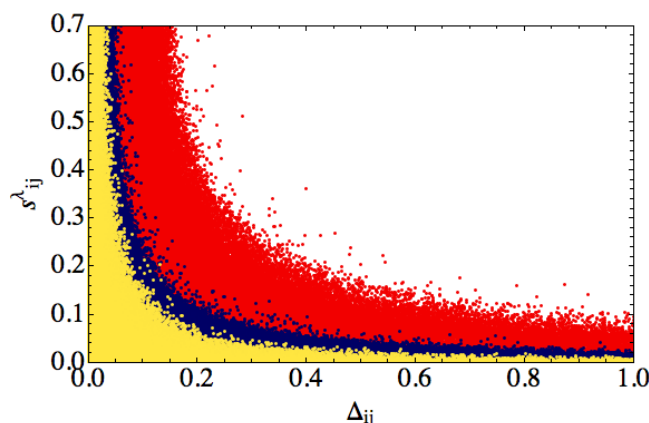
Figure 5. Allowed ranges for the mixing angles s_{ij}^\lambda as a function of the deviation from the ij -degeneracy line \Delta_{ij} = |D_{\lambda,ii} - D_{\lambda,jj}| . ij = 12 in yellow, ij = 13 in blue, ij = 23 in red.
