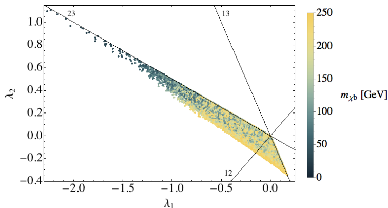
Figure 14. Allowed region in the \lambda_1 - \lambda_2 -plane for the quasi-degeneracy scenario, after imposing the relic abundance, LUX and flavor constraints. The DM mass m_{\chi_b} is indicated by the color, and the ij -degeneracy lines are sketched.
