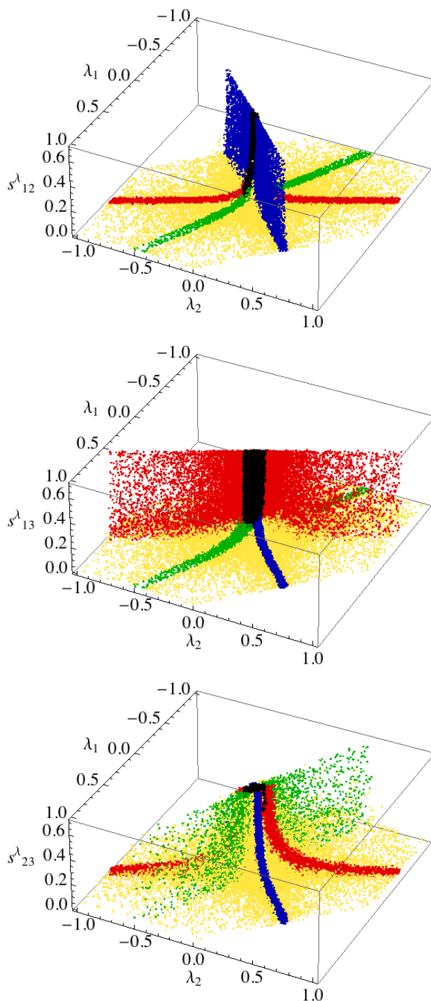
Figure 4. Scenarios for the structure of \lambda : universality (black), 12-degeneracy (blue), 13-degeneracy (red), 23-degeneracy (green), small mixing (yellow).
