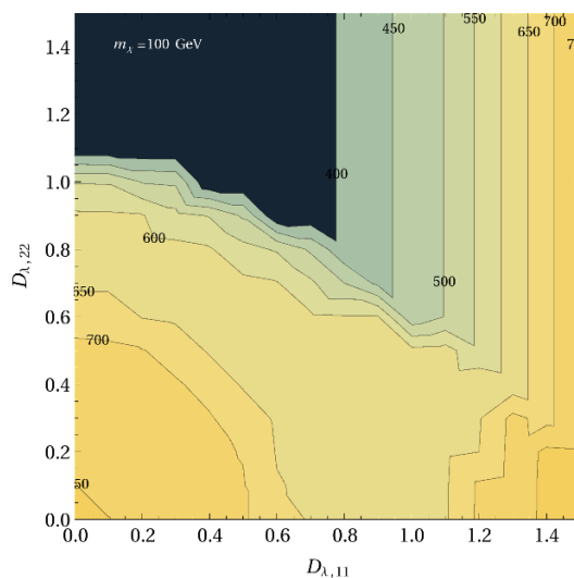
Figure 16. Exclusion contours for m_\phi (in GeV) for various values of D_{\lambda,11} and D_{\lambda,22} from the CMS sbottom [66] and squark [67] searches, obtained for the NLO estimate. D_{\lambda,33} is fixed by the relic abundance constraint.
