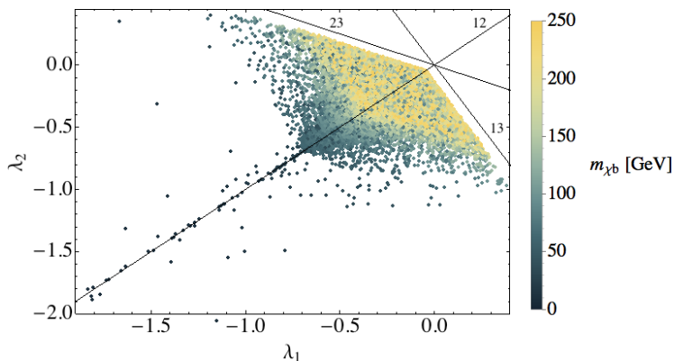
Figure 9. Allowed region in the \lambda_1 - \lambda_2 -plane for the single flavor freeze-out scenario, after imposing the relic abundance, LUX and flavor constraints. The DM mass m_{\chi_b} is indicated by the color, and the ij -degeneracy lines are sketched.
