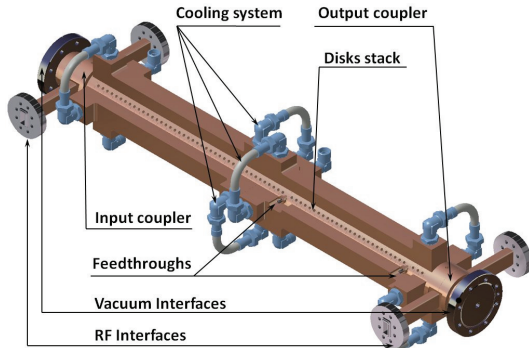
Figure 1: General view of accelerating structure.
