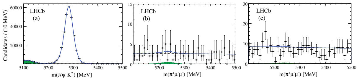
FIG. 2 (color online). Invariant mass distributions with fits overlaid of candidate mass spectra for (a) J/\psi K^- , (b) \pi^+ \mu^- \mu^- ( \mathcal{S} ), and (c) \pi^+ \mu^- \mu^- ( \mathcal{L} ). Backgrounds are (green) shaded; they peak under the signal in (b) and (c). The dotted lines show the combinatorial backgrounds only. The solid line shows the sum of both backgrounds.
