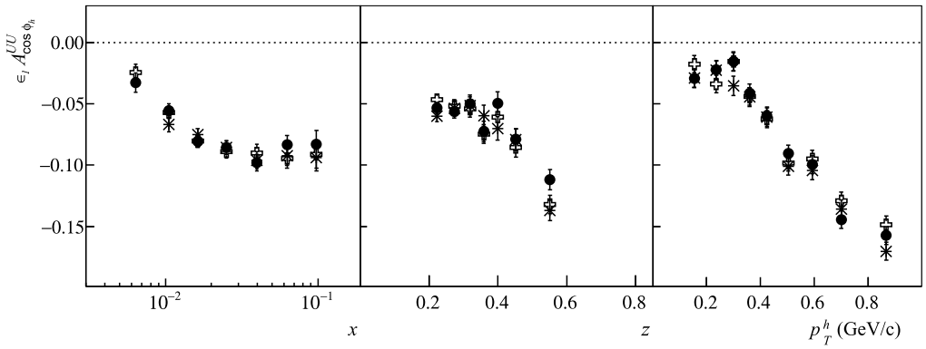
Fig. 8. The amplitudes of the \cos \phi_h modulations ( \epsilon_1 A_{\cos \phi_h}^{UU} ) for positive hadrons extracted using the acceptance corrections from the three Monte Carlo samples of Fig. 7.
