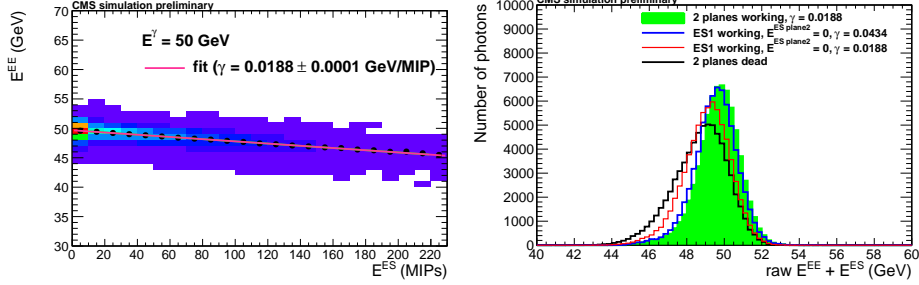
Figure 2: Left: Energy measured by EE crystals versus the energy deposits in ES (in units of the energy lost by minimum ionising particles (MIPs) in ES) by using MC unconverted 50 GeV photons with |\eta| between 1.7 and 2.3. Right: The combined EE + ES energy distribution for both planes working (green) and for both ES planes dead (black). In red, the resolution if only ES1 is working, but incorrectly using the gamma for the both planes working. In blue, the resolution obtained for ES1 working, but ES2 dead, using the correct \gamma obtained from the dead channel calibration method.
