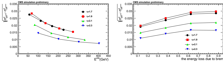
Figure 1: Left: The improvement of the new energy clustering for different \eta values. Right: The improvement of the new energy clustering for different fractions of energy loss due to bremsstrahlung.
