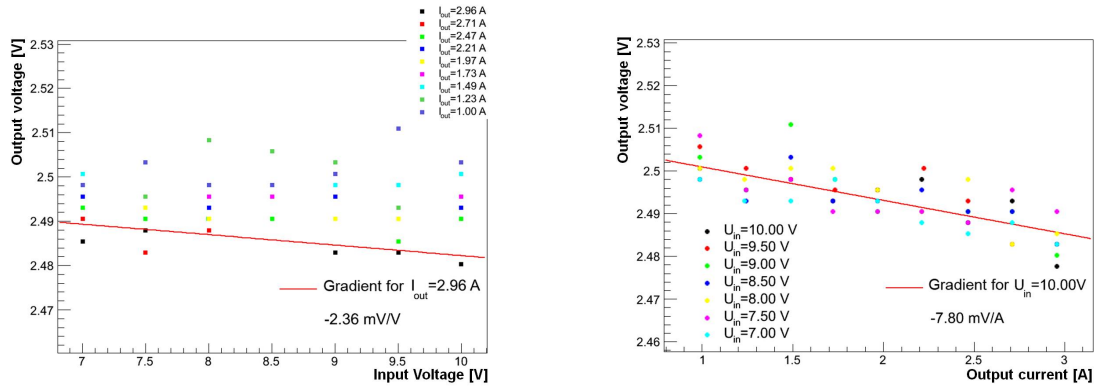
Figure 6. Line regulation (left) and load regulation (right) of a PIX_V9 DC-DC converter with 2.5 V output voltage. The red lines represent linear fits.
