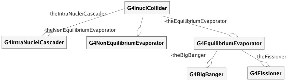
Figure 2.2: General relationships with Bertini cascade classes. Sub-model management is handled by the G4InuclCollider class (for details see Listing 2.2) [72].
