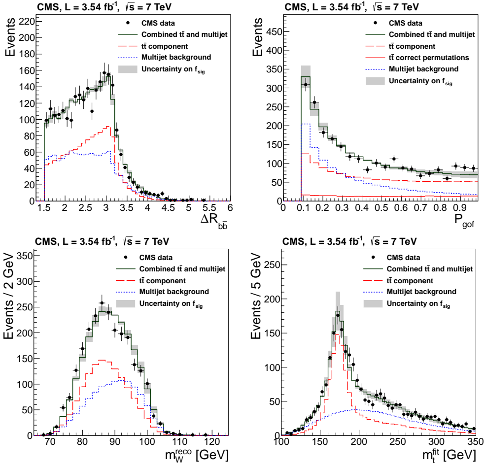
Figure 1: Distance \Delta R_{b\bar{b}} between the two bottom-quark candidates (top left), probability of the kinematic fit (top right), reconstructed top-quark mass from the kinematic fit (bottom right), and average reconstructed W-boson mass before being constrained by the kinematic fit (bottom left). The simulated t\bar{t} signal ( m_{t,\text{gen}} = 172.5 \text{ GeV} ) and background from event mixing are normalized to data with an uncertainty band from the signal fraction f_{\text{sig}} .
