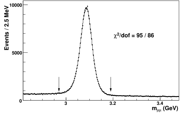
FIG. 13: Top: Fractional momentum correction \Delta p/p as a function of the mean inverse transverse momentum of the muons from J/\psi decay. Bottom: Representative m_{\mu\mu} fit (histogram) to data (circles), here in the range \langle 1/p_T^\mu \rangle = (0.2, 0.225) \text{ GeV}^{-1} . The fit region is indicated by arrows.
