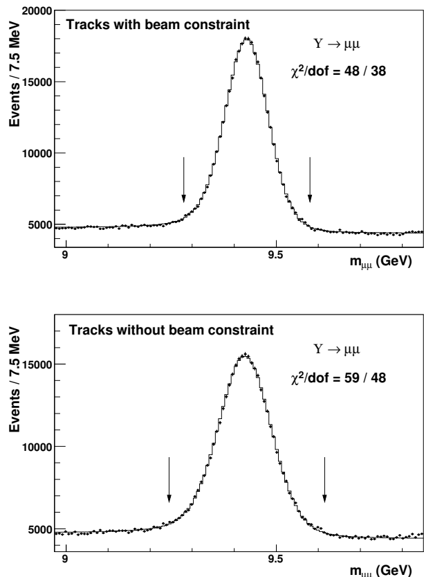
FIG. 15: Distribution of m_{\mu\mu} for the best-fit templates (histograms) and the data (circles) in the \Upsilon \rightarrow \mu\mu sample used to calibrate the muon momentum scale. The muon tracks are reconstructed with (top) or without (bottom) a constraint to the beam position in the transverse plane. The arrows enclose the fit region.
