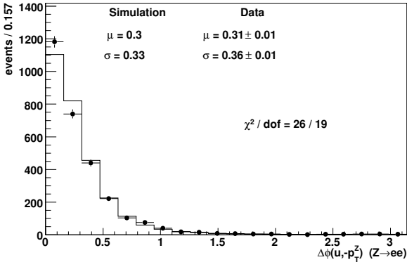
FIG. 32: Distributions of the angular separation between the reconstructed recoil vector \vec{u}_T and the dilepton -\vec{p}_T^{\ell\ell} vector in Z \rightarrow ee decays, for simulation (lines) and data (circles) respectively. The distributions are shown for the ranges p_T^{\ell\ell} < 8 GeV (top), 8 < p_T^{\ell\ell} < 15 GeV (middle), and p_T^{\ell\ell} > 15 GeV (bottom).
