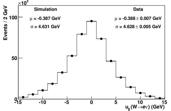
FIG. 33: Distributions of u_{||} from simulation (histogram) and data (circles) for W boson decays to \mu\nu (top) and e\nu (bottom) final states. The simulation uses parameters fit from Z boson data, and the uncertainty on the simulation is due to the statistical uncertainty on these parameters. The data mean ( \mu ) and rms spread ( \sigma ) are well-modeled by the simulation.
