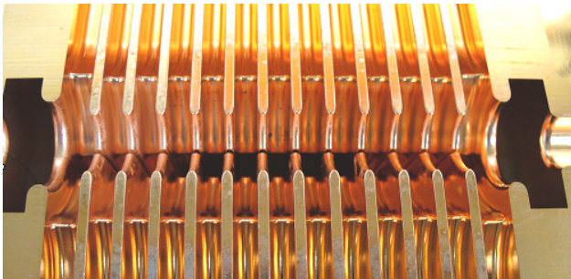
Figure 1: Photo showing bottom two quadrants of the HDX structure after testing. There are slots between the regular irises but not the matching cell irises on each end.
