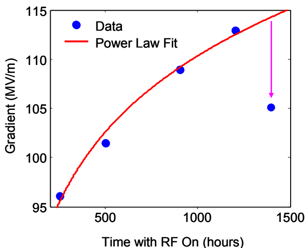
Figure 3: CERN/KEK/SLAC T18 disk structure gradient over time with 230 ns pulses and a breakdown rate of 2 \times 10^{-6} pulse per meter.
