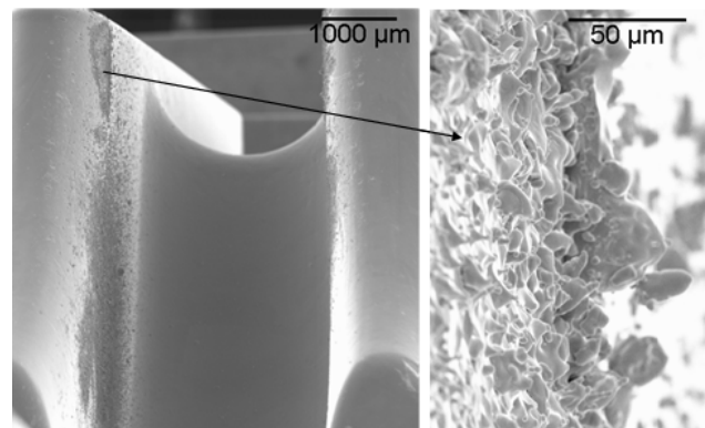
Figure 2: SEM Photo of a HDX cell 7 quadrant after the run. The right photo is a blowup of the triangular patch on the left, showing the growth of melted nodules.
