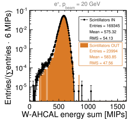
Figure 20: Energy sum distributions for 20 GeV e^+ , before (left) and after selection (right). Two runs taken with and without beam line scintillators are compared.
