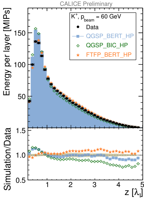
Figure 53: Longitudinal profile from shower start for 60 GeV K^+ . The data are compared with the GEANT4 physics lists. In the lower part of the figure, the ratios between simulation and data are shown. The grey band indicates the systematic uncertainties on data.
