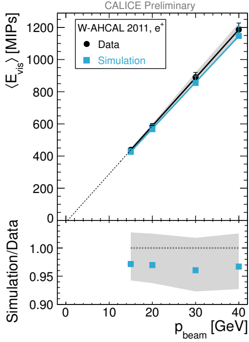
Figure 24: Dependence of the mean visible energy on the beam momenta for 2011 e^+ W-AHCAL data. The grey band shows the overall uncertainty. The lines indicate fits with the function E_{\text{vis}} = u + v \cdot p_{\text{beam}} .
