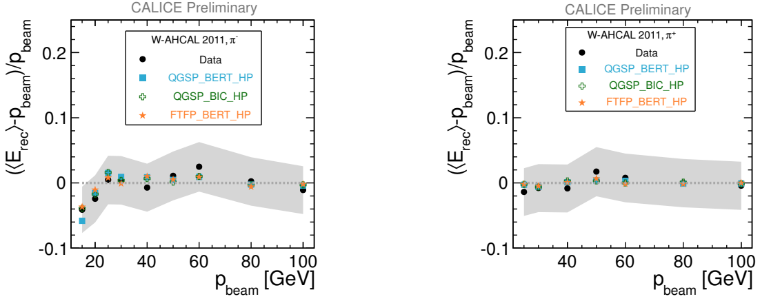
Figure 30: Deviations from linearity for the W-AHCAL 2011 \pi^- (left) and \pi^+ (right) data. The data are compared with the selected GEANT4 physics lists. The grey band shows the overall uncertainty.
