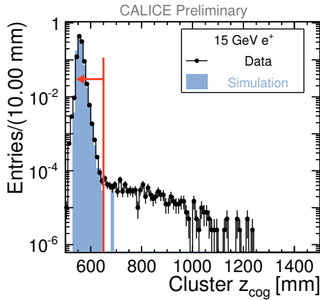
Figure 16: Distribution of the cluster centre-of-gravity in z (in the laboratory system) for 15 GeV e^+ . The line indicates the selection cut.
