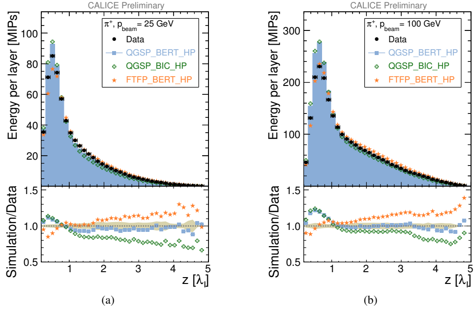
Figure 34: Longitudinal profiles from shower start for 25 GeV (a) and 100 GeV \pi^+ (b). In the lower part of the figures, the ratio between the GEANT4 physics lists and data is shown. The grey band indicates the systematic uncertainties on data.
