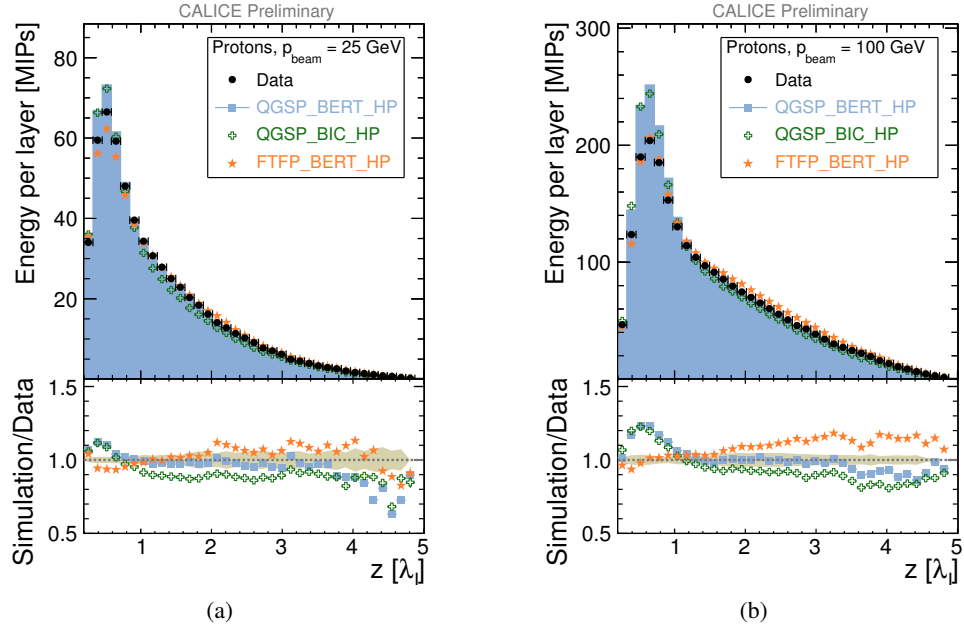
Figure 45: Longitudinal profiles from shower start for 25 GeV (a) and 100 GeV (b) protons. In the lower part of the figures, the ratio between the GEANT4 physics lists and data is shown. The grey band indicates the systematic uncertainties on data.
