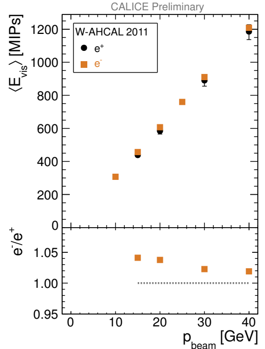
Figure 22: Average e^\pm visible energy as a function of the beam momentum.
