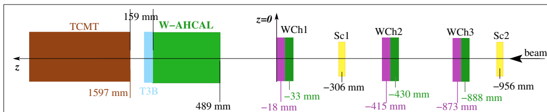
Figure 1: Sketch of the CERN 2011 test beam line as implemented in the Mokka model TBCern2011WAHCAL (not to scale), where Sc stands for scintillator and WCh for wire chamber. The beam enters from right.
