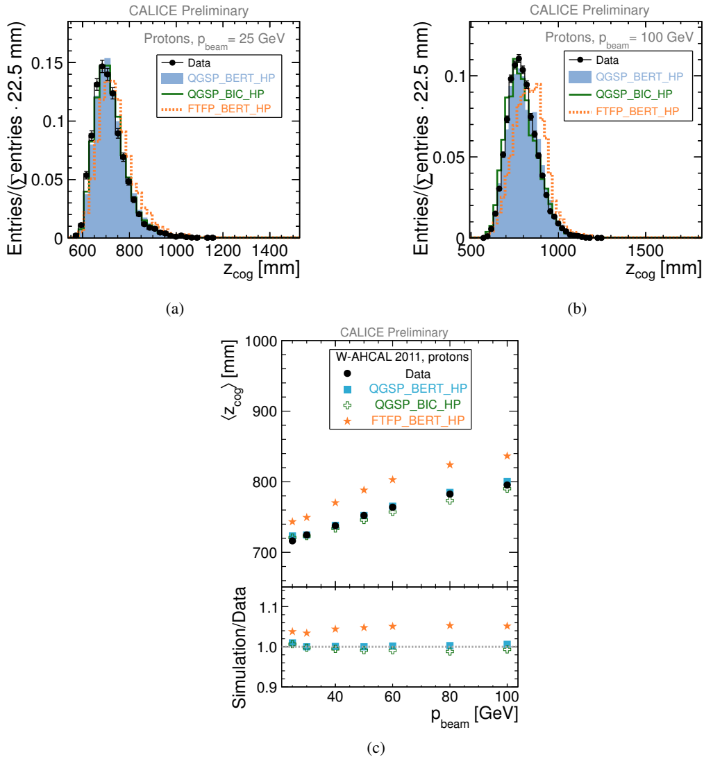
Figure 46: Distribution of the centre-of-gravity in z for 25 GeV (a) and 100 GeV protons (b). Dependence of mean centre-of-gravity in z on the beam momentum (c). The data are compared with the GEANT4 physics lists.
