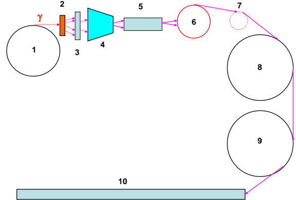
Figure 1: Layout of the Compton based positron source. 1: Compton ring; 2: conversion target; 3: positron selection; 4: adiabatic matching device; 5: pre-accelerator; 6: stacking ring; 7: time diagram transformer; 8: pre-damping ring; 9: damping ring; 10: main accelerator.
