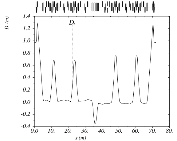
Figure 4: SR first-order dispersion for a single super period.
