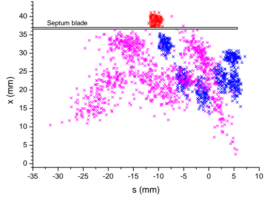
Figure 6: Beam particles at injection (red symbols), on the first couple of turns (blue symbols), and at the end of the first synchrotron period (magenta symbols).
