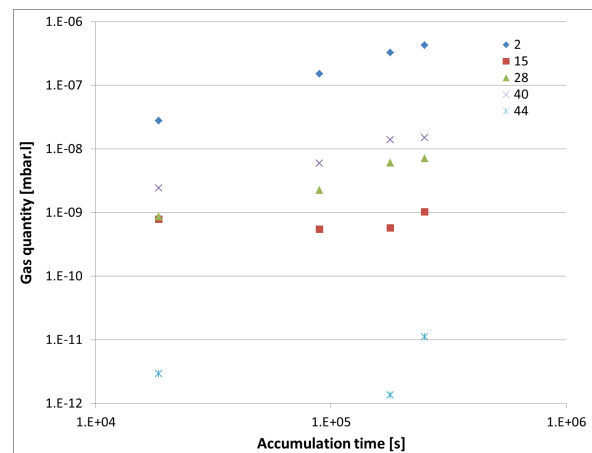
Figure 2 Accumulated gas as a function of time for different species.
