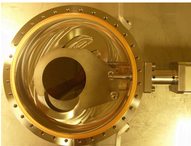
Figure 1: Picture of the fast valve partially opened.
