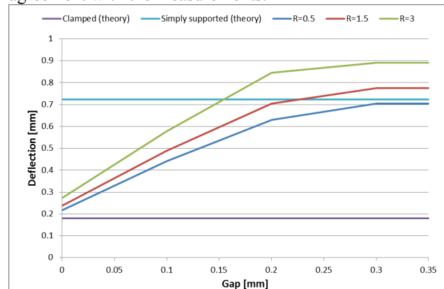
Figure 4: Estimation of the deflection under vacuum for different geometrical parameters.
