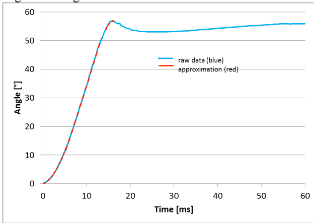
Figure 3 Measures and approximation of the angle as a function of time during the closing.
