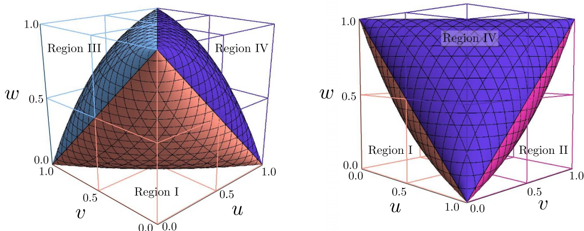
Figure 1. Illustration of Regions I, II, III and IV. Each region lies between the colored surface and the respective corner of the unit cube.
