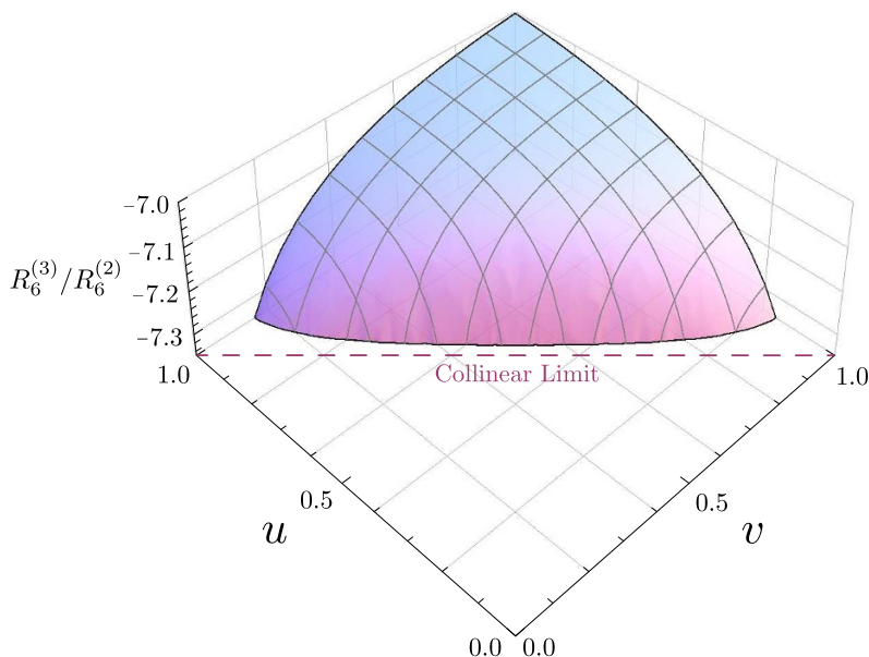
Figure 9. The ratio R_6^{(3)}(u, v, w)/R_6^{(2)}(u, v, w) on the plane u + v - w = 1 , as a function of u and v .
