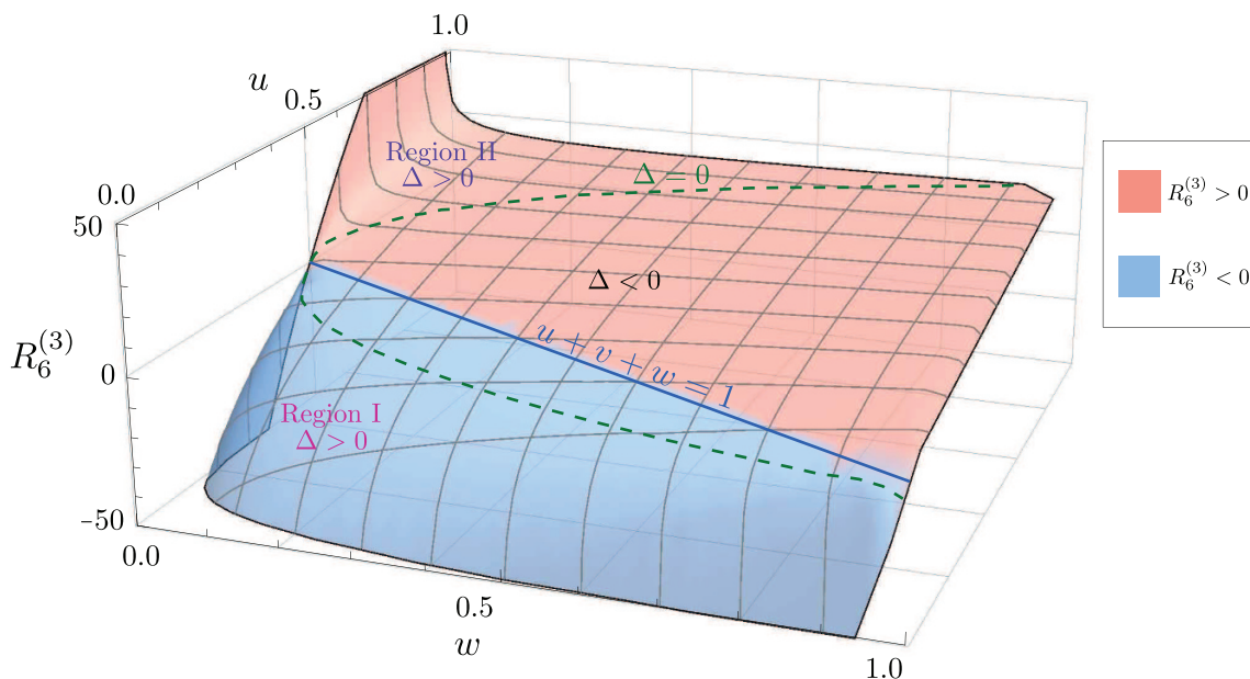
Figure 11. Plot of R_6^{(3)}(u, v, w) on the plane u = v , as a function of u and w . The region where R_6^{(3)} is positive is shown in pink, while the negative region is blue. The border between these two regions almost coincides with the intersection with the u + v + w = 1 plane, indicated with a solid line. The dashed parabola shows the intersection with the \Delta = 0 surface; inside the parabola \Delta < 0 , while in the top-left and bottom-left corners \Delta > 0 .
