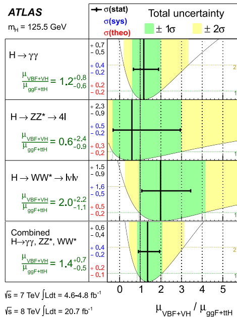
Fig. 8. Measurements of the \mu_{VBF+VH}/\mu_{ggF+ttH} ratios for the individual diboson final states and their combination, for a Higgs boson mass m_H = 125.5 GeV. The best-fit values are represented by the solid vertical lines, with the total \pm 1\sigma and \pm 2\sigma uncertainties indicated by the dark- and light-shaded band, respectively, and the statistical uncertainties by the superimposed horizontal error bars. The numbers in the second column specify the contributions of the statistical uncertainty (top), the total (experimental and theoretical) systematic uncertainty (middle), and the theoretical uncertainty (bottom) on the signal cross section (from QCD scale, PDF, and branching ratios) alone. For a more complete illustration, the distributions of the likelihood ratios from which the total uncertainties are extracted are overlaid.
