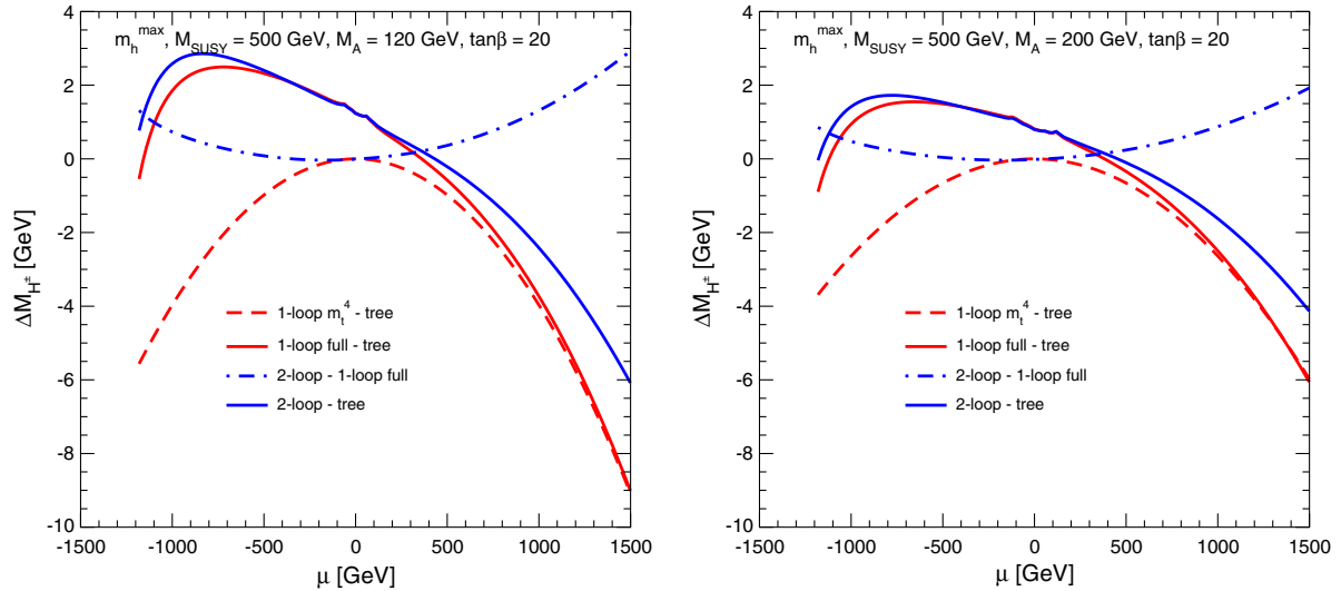
FIG. 12 (color online). \Delta M_{H^\pm} := M_{H^\pm} - m_{H^\pm} and M_{H^\pm}^{2\text{-loop}} - M_{H^\pm}^{1\text{-loop}} are shown for M_A = 120 GeV (left) and M_A = 200 GeV (right plot), \tan\beta = 20 and M_{\text{SUSY}} = 500 GeV as a function of \mu in the m_h^{\text{max}} scenario. M_{H^\pm} is evaluated at the two-loop level (blue/dark gray solid). Also shown are the corresponding one-loop results of \mathcal{O}(m_t^4/M_W^2) (dashed), the full one-loop corrections (red/light gray solid) and the difference between the two-loop and the full one-loop result (dot-dashed).
