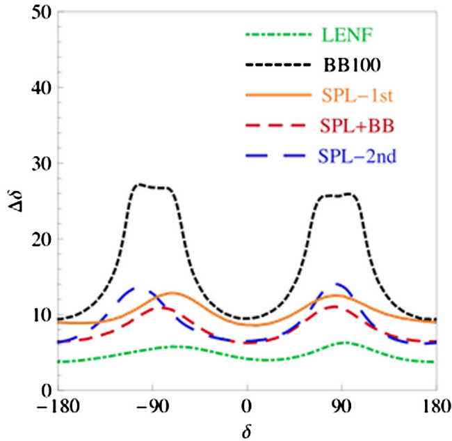
FIG. 25. The 1\sigma measurement errors for the CP angle \delta as a function of \delta . The facilities studied are as follows. LENF: the Low Energy Neutrino Factory, with a 10 GeV muon energy, 1.4 \times 10^{21} decays per year and a single 100 kt mass magnetized iron neutrino detector (MIND) at a baseline of 2000 km; BB100: a \gamma = 100 Beta Beam, with 1.3/3.5 \times 10^{18} decays per year of Ne/He and a 500 kt water Cherenkov detector (MEMPHYS) at Fréjus; SPL-1st: a 4 MW SPL Super Beam with 500 kt water Cherenkov detector at Fréjus, corresponding approximately to the first oscillation maximum; SPL-2nd: as above, but with the detector at Canfranc, corresponding to approximately the second oscillation maximum; SPL + BB: the combination of BB100 and SPL-1st.
