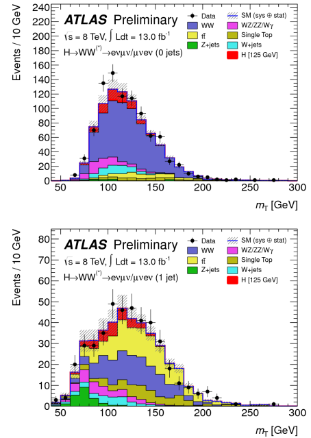
Figure 5. m_T distribution in the zero (one) jet bin after all signal selection cuts in the top (bottom) plot [2]. The expectation for a 125 GeV Higgs signal is shown in red.
