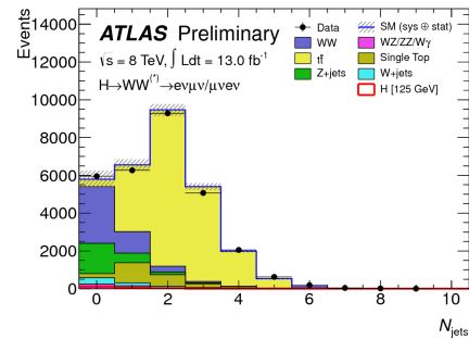
Figure 1. The jet multiplicity distribution after signal pre-selection cuts are applied [2].
