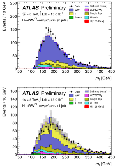
Figure 4. The m_T distribution in the WW zero (one) jet CR is shown in the top (bottom) plot. The WW rate predicted by Monte Carlo simulation has not yet been normalized to the data. The top backgrounds have been normalized according to the procedure described in the text [2].
