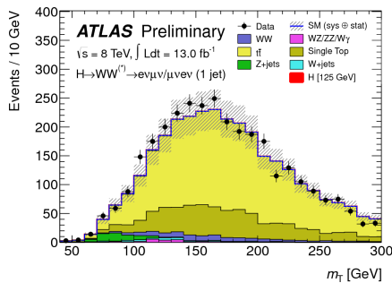
Figure 3. m_T distribution in the top one jet control region. The rate predicted by Monte Carlo simulation has not yet been normalized to the data. [2]
