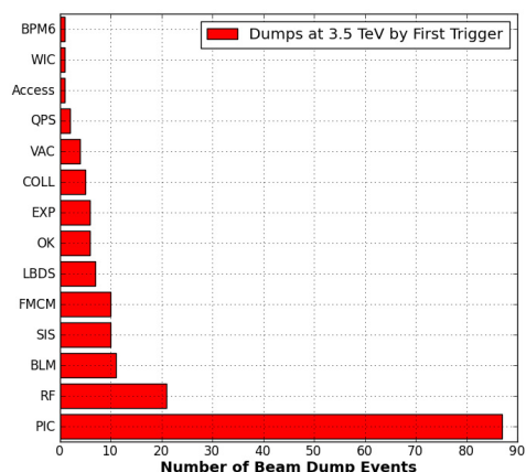
Figure 12: Breakdown by first trigger of beam dumps at 3.5 TeV for all fills in the 2011 Proton Run where a non-programmed dump occurred which was not classified as having a Machine Protection beam dump cause of End-of-Fill.
