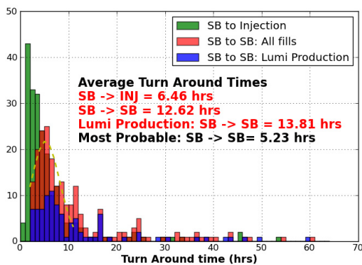
Figure 6: Turn around time for fills during the 2011 Proton Run. The Luminosity production phase is defined as fills with 1380 bunches per beam injected.
