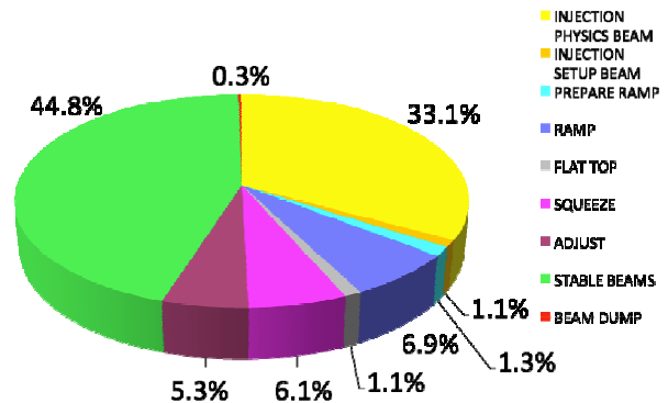
Figure 11: Breakdown by beam mode of non-programmed beam dumps that occurred in the 2011 Proton Run.
