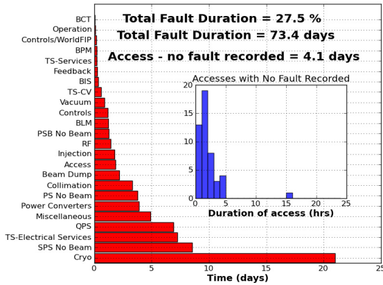
Figure 8: Breakdown of LHC downtime by system as registered in the e-logbook fault tracking. The inset shows the distribution of downtime events where no fault was recorded in the e-logbook, but for which the machine was in a state compatible for access.
