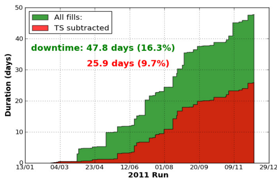
Figure 9: Total cryogenics downtime as a function of the run duration. Downtime is defined as the absence of the global AND of all the Cryo_Maintain signals.
