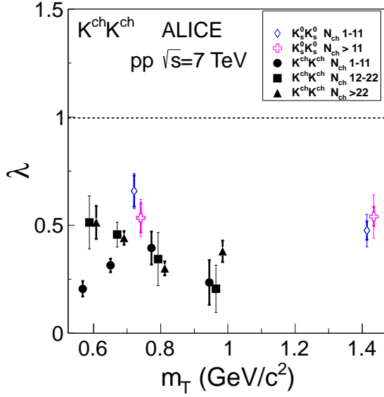
Fig. 3: \lambda -parameters of K^{\text{ch}}K^{\text{ch}} versus m_T extracted by fitting correlation functions shown in Fig. 2 to Eq. (1) and the baseline to Eq. (2). For comparison the K_S^0 K_S^0 [10] \lambda -parameters measured by ALICE in 7 TeV pp collisions are also shown. Statistical (darker lines) and total errors are shown. The points corresponding to the second and third multiplicity bins are offset by 0.03 \text{ GeV}/c^2 for clarity.
