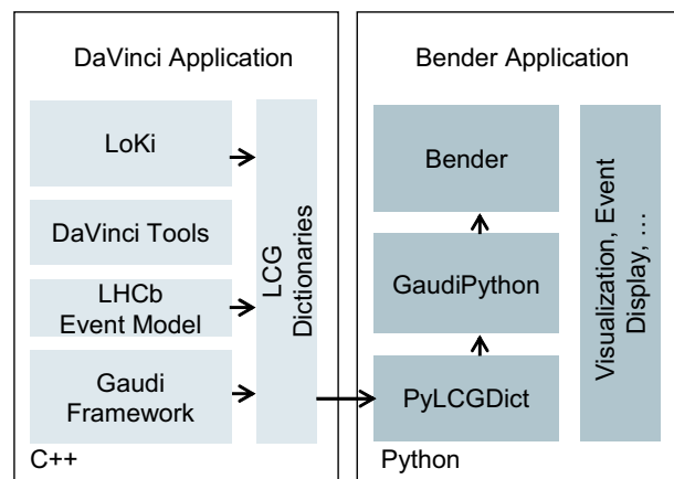
Figure 1: The schematic relations between the DAVINCI and BENDER frameworks
