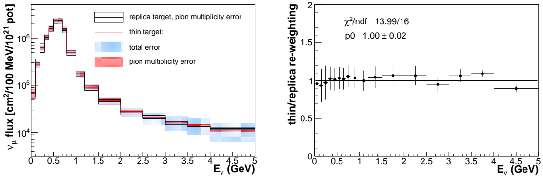
Fig. 21: Re-weighted \nu_\mu flux predictions at the far detector of T2K based on the NA61 thin-target and replica-target data [left] and ratio of the two predictions [right]. Details about the associated errors are given in the text. A linear fit to the ratio [right] is shown by the solid line.
