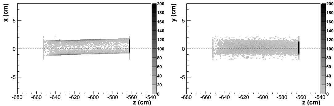
Fig. 13: Distribution of the point of closest approach of the TPC tracks in the x-z [left] and y-z [right] projections after backward extrapolation to the surface of the target. The fact that the side of the target appears fuzzy in the vertical projection ( y ) is a consequence of the azimuthal acceptance of the detector (see Fig. 7) which is further constrained by the \pm 30 degree wedge cut defined in the text.
