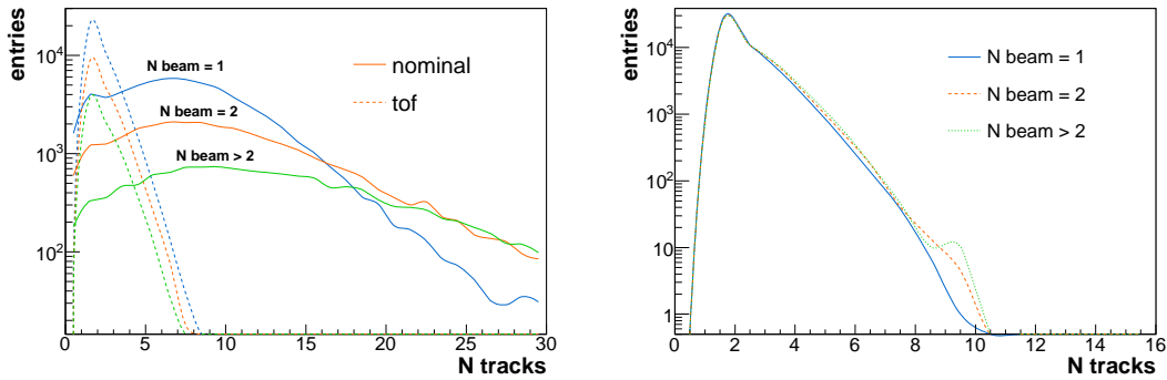
Fig. 9: Track multiplicity in the TPCs without (solid) and with (dashed) the ToF-F requirement for events with different numbers of beam particles [left]. Multiplicity distributions normalised to the number of single beam particle events with the ToF-F requirement [right].
