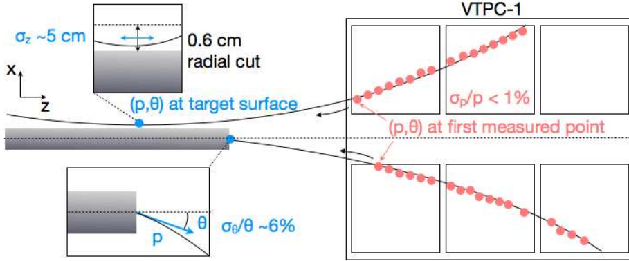
Fig. 10: Sketch depicting the backward extrapolation of TPC tracks onto the surface of the target. The point of closest approach is determined and the track parameters p and \theta are calculated at this point. Only tracks for which this point lies within a distance of 0.6 cm around the target surface are accepted. The resolution for the different track parameters are also given in the figure.
