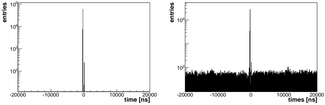
Fig. 8: Time distribution of beam particles in a 40 \mu\text{s} time window for single beam particle events [left] ( \sim 60\% of all events), and events with two beam particles [right] ( \sim 40\% of all events). The beam time is centered at -300 ns.
