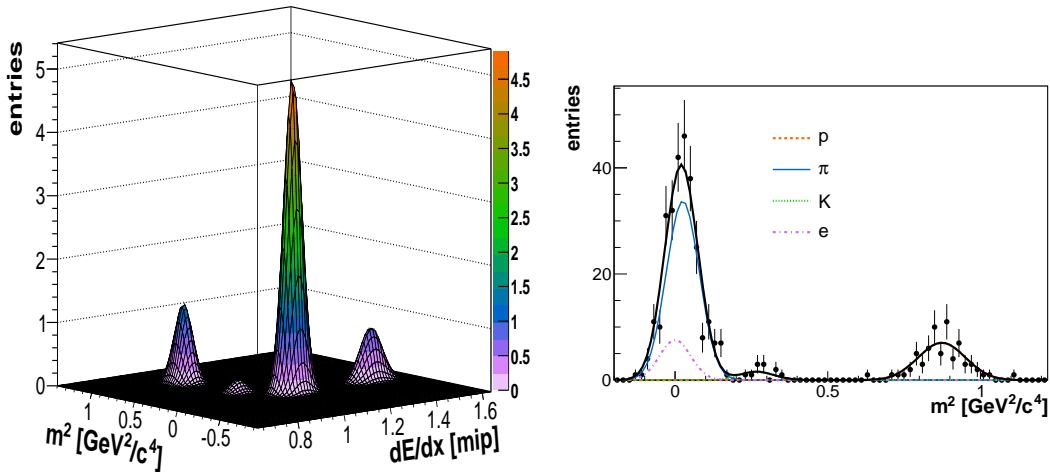
Fig. 15: Two-dimensional fit of the data in the (m^2, dE/dx) plane [left] and respective mass squared projection [right], for 40 < \theta < 100 mrad and 2.4 < p < 3.2 GeV/c at the surface of the target. The different components of the fit are shown with different line styles.
