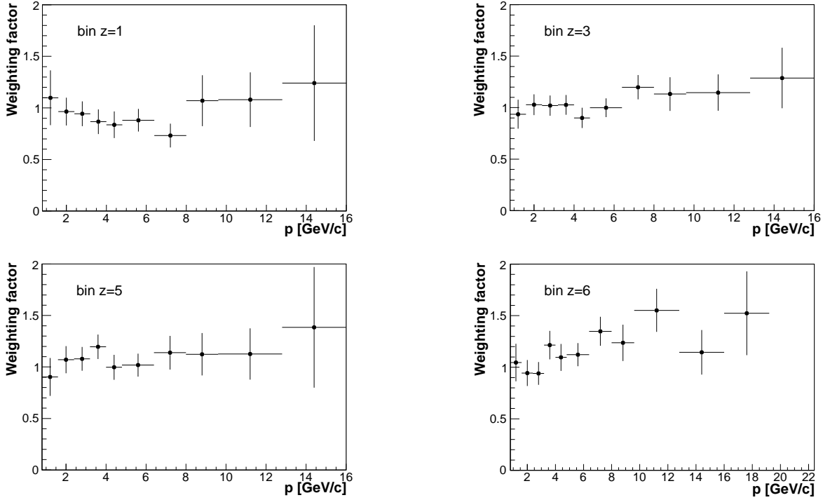
Fig. 20: Re-weighting factors for outgoing positively charged pions in the angular interval [40-100] mrad for the most upstream [top left], central [top right] and most downstream [bottom left] longitudinal bins, and in the angular interval [0-40] mrad for the downstream face of the target [bottom right]. Error bars correspond to the sum in quadrature of statistical and systematic uncertainties.
