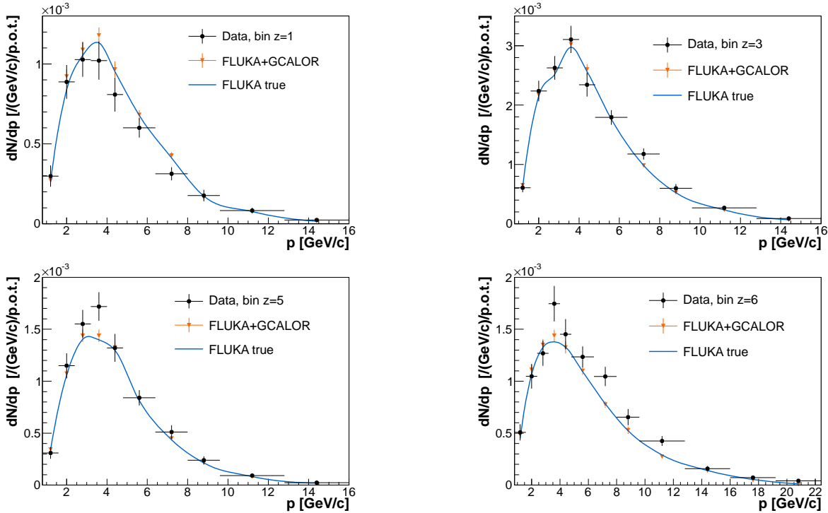
Fig. 19: Spectra of outgoing positively charged pions normalised to the momentum bin size and number of protons on target in the angular interval [40-100] mrad for the most upstream [top left], central [top right] and most downstream [bottom left] longitudinal bins, and in the angular interval [0-40] mrad for the downstream face of the target [bottom right]. Error bars correspond to the sum in quadrature of statistical and systematic uncertainties. Smooth curves show the prediction of FLUKA2011.2 associated to tracks reconstructed within the acceptance of the NA61 detector (described in Section 3.4). FLUKA+GCALOR refers to the MC yields after reconstruction and PID analysis.
