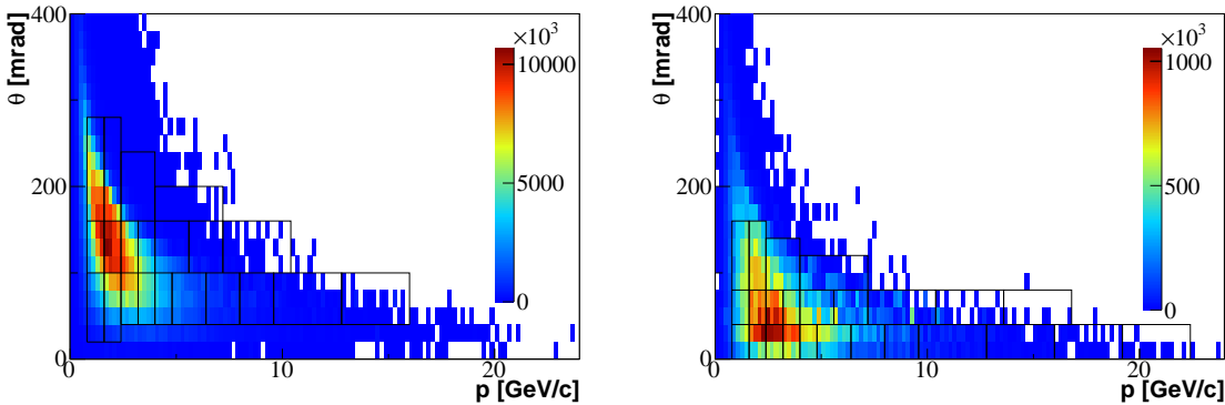
Fig. 6: Kinematical phase space of positively charged pions (for 10^{21} pot) exiting from the side of the target [left] or from the downstream face [right], and producing neutrinos in the direction of the far detector of T2K. The respective analysis binning of the NA61 data with the replica of the T2K target is overlaid on top. Predictions obtained from the T2K beam simulation.
