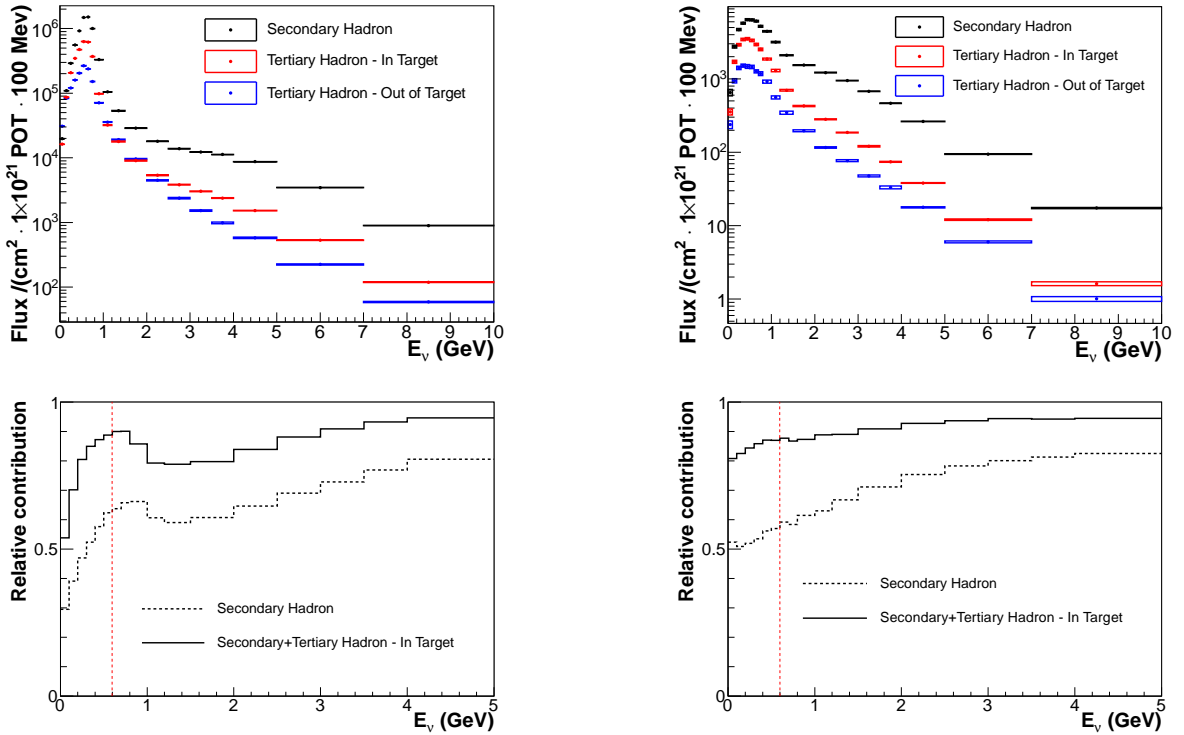
Fig. 2: Secondary and tertiary components of the \nu_\mu [top left] and \nu_e [top right] fluxes at the far detector. The contribution of parents originating from the target sums up to 90 %, among which 60 % are due to the secondary component and 30 % due to re-interactions in the target (the in-target component). The relative contributions of the secondary and total in-target (secondary+tertiary in-target) components are shown for \nu_\mu [bottom left] and \nu_e [bottom right] as a function of energy. The dashed vertical line shows the location of the peak of the beam energy spectrum (600 MeV). Predictions are based on FLUKA2008.3b and re-weighted by the NA61 thin-target data.
