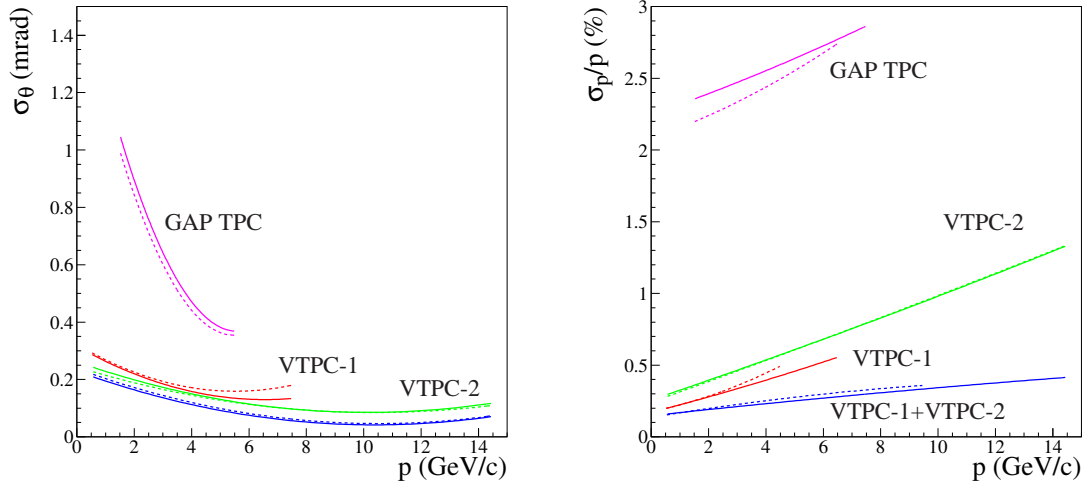
Fig. 11: Error on the polar angle [left] and momentum resolution [right] as a function of momentum of the TPC tracks for data (solid) and MC (dashed). Labels refer to track topologies defined in the text.
