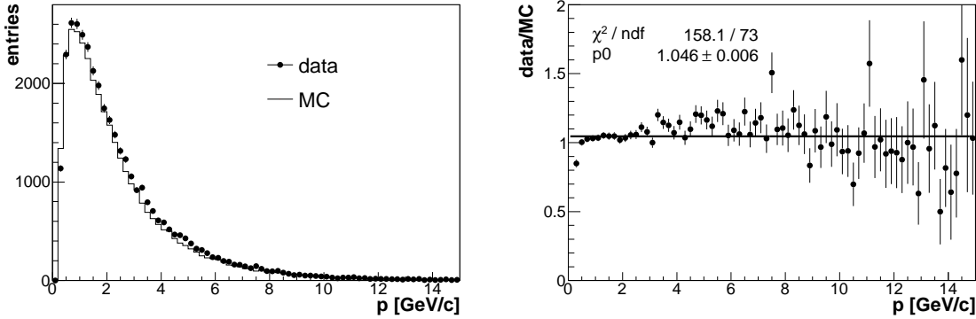
Fig. 17: Momentum distribution of negatively charged pion-like tracks [left] after backward extrapolation, requirement for a point of closest approach closer than 0.6 cm to the surface of the target and a simple dE/dx -based PID selection to reject electrons. A first-order polynomial fit to the ratio of data to MC [right] returns a constant of 1.046.
