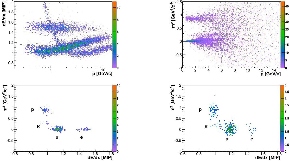
Fig. 14: Top panel: dE/dx [left] and mass squared [right] distributions for all TPC tracks as a function of the track momentum at the first fitted TPC cluster. Bottom panel: (m^2, dE/dx) distributions of positively charged tracks for 40 < \theta < 100 mrad polar angle and 2.4 < p < 3.2 GeV/c [left], 4 < p < 4.8 GeV/c [right] momentum at the surface of the target.
