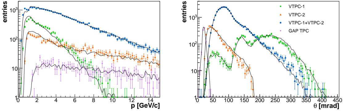
Fig. 16: Distributions of momentum [left] and polar angle [right] of TPC tracks at the surface of the target for data (coloured markers) and MC (solid smoothed curves). The different track topologies are specified in the legend on the right plot and described in the text.
