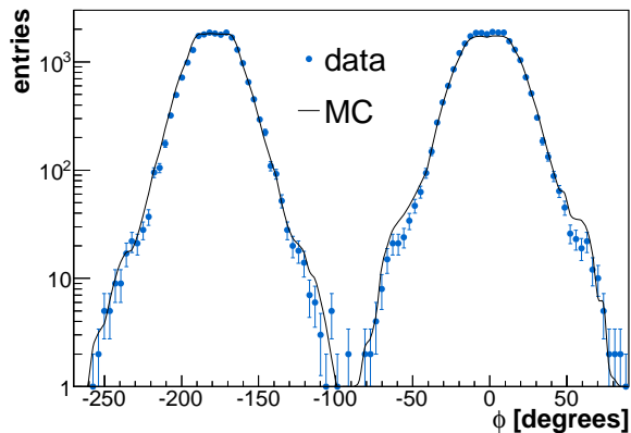
Fig. 7: Distribution of the azimuthal angle, \phi , of all TPC tracks in data (markers) and MC (line).
