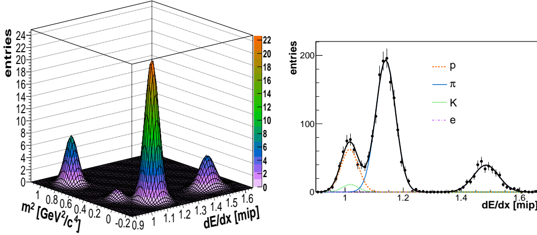
Fig. 18: Two-dimensional fit of the simulated data in the (m^2, dE/dx) plane [left] and respective dE/dx projection [right], for 40 < \theta < 100 mrad and 2.4 < p < 3.2 GeV/c at the surface of the target. The different components of the fit are shown with different line styles.
