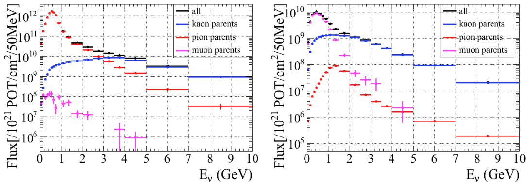
Fig. 1: Prediction (based on FLUKA2008.3b and re-weighted by the NA61 thin target data) of the \nu_\mu [left] and \nu_e [right] fluxes at the near detector of T2K. Different colours refer to the contributions of the various parent particles.
