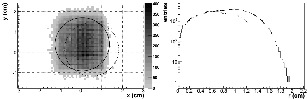
Fig. 12: Profile [left] and radial distribution [right] of the beam on the upstream face of the replica target. The radial distribution is shown before (solid) and after (dashed) applying a beam track selection defined in the text below. The solid (dashed) circle shows the position of the upstream (downstream) face. The dotted vertical line shows the radius of the target.
