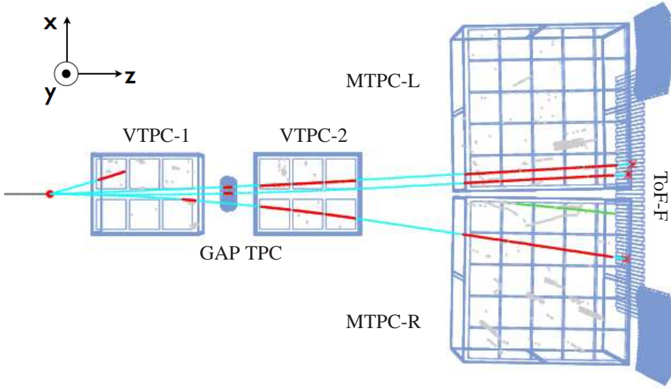
Fig. 4: An example of a reconstructed p+C interaction at 30 GeV beam energy in the replica of the T2K target showing tracks reconstructed in the TPCs and associated with hits in the ToF-F detector. The incoming beam direction is along the z axis. The magnetic field bends the trajectory of outgoing charged particles in the x - z (horizontal) plane. The drift direction in the TPCs is along the y axis.
