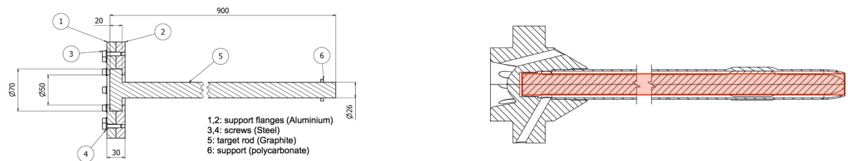
Fig. 5: Technical drawing (side view) of the replica target used during the NA61 data taking [top left] consisting of a 90 cm long graphite rod and aluminium support flanges. Drawing of the complete geometry of the T2K target [top right]. The overlaid red rectangle represents the simplified geometry of the replica target. View of the T2K target and its cooling envelope embedded in the first focusing horn of the T2K beam line [bottom].
