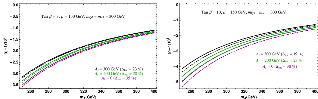
Figure 5. (r_t - 1) as a function of m_A for \tan\beta = 3 (left) and \tan\beta = 10 (right). In addition to the stop-higgsino loop with parameters A_t and \mu as shown, a sbottom-gluino contribution is also included with m_{D3} = 300 GeV, M_{\tilde{g}} = 800 GeV. The solid curves are derived by using the value of r_b , extracted from FeynHiggs, in our formula eq. (3.5). The dashed curves are derived using FeynHiggs. Similar results are found for r_V .
