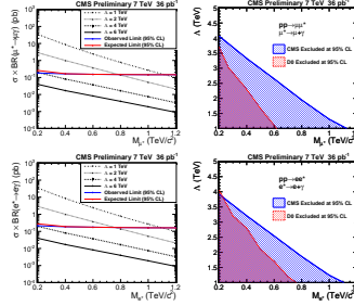
Figure 1. Left: Observed (blue) and predicted (red) limits on the excited muon (top) and electron (bottom) production cross section times branching ratio at 95% CL, as functions of the excited lepton mass. Right: The region in the (\Lambda, M_{\ell^*}) plane excluded at the 95% CL by the present search, both for muons (top) and electrons (bottom).
