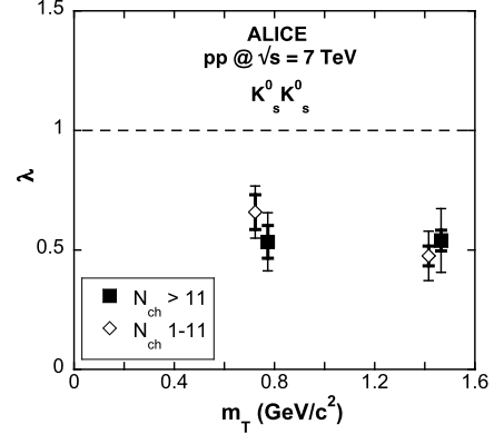
Fig. 6. \lambda parameters extracted by fitting the Lednicki parametrization to K_s^0 K_s^0 correlation functions as shown in Fig. 5. Statistical (darker lines) and total uncertainties are shown. The N_{\text{ch}} > 11 points are offset by 0.05 \text{ GeV}/c^2 for clarity.
