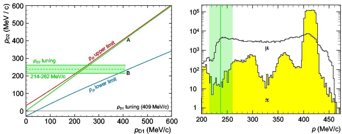
Figure 4. Working principle of the MICE beam line. Left-hand panel: the red and blue lines are the kinematic limits of the spectrum for muons produced in pion decays. By tuning D2 to the backward going muon peak an almost pion-free sample is produced. Right-hand panel: simulation showing pion and muon spectra at the end of the decay solenoid. Only high momentum pions survive. The green band shows the acceptance of D2, when tuned to the backward-going muon peak.
