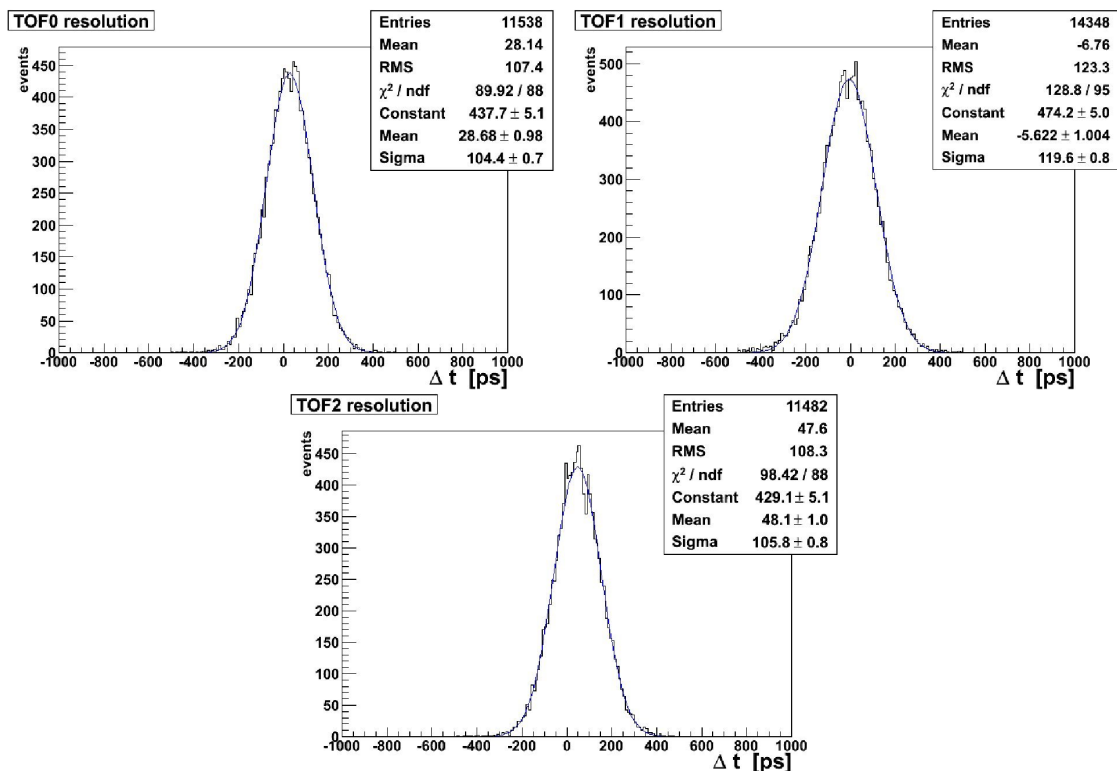
Figure 15. Time difference \Delta t_{xy} between vertical and horizontal slabs in TOF0, TOF1 and TOF2. The trigger is on TOF1.
