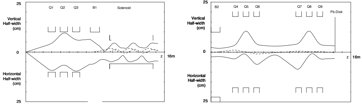
Figure 11. MICE beam-line envelope for the baseline case with \varepsilon_N = 6\pi \text{ mm} \cdot \text{rad} and p_z = 200 \text{ MeV}/c . Left panel: pion optics for the upstream section. Right panel: muon optics for the downstream section. The lead scatterer (“diffuser”) used in this simulation for practical reasons has been realized using brass and tungsten. For both panels the top half of the plot shows the vertical envelope and the bottom half shows the horizontal envelope.
