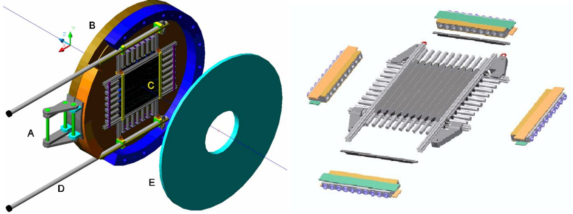
Figure 14. Shielding used for TOF PMTs. Left panel: TOF1 global cage showing, A) extraction brackets, B/E) shielding plates, C) TOF1 detector in working position, D) rails to move TOF1 outside the shielding cage. Right panel: TOF2 local shielding with massive soft iron boxes.
