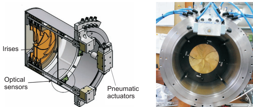
Figure 10. Left panel: schematic of the MICE diffuser showing the irises. Right panel: one of the brass irises being tested.
