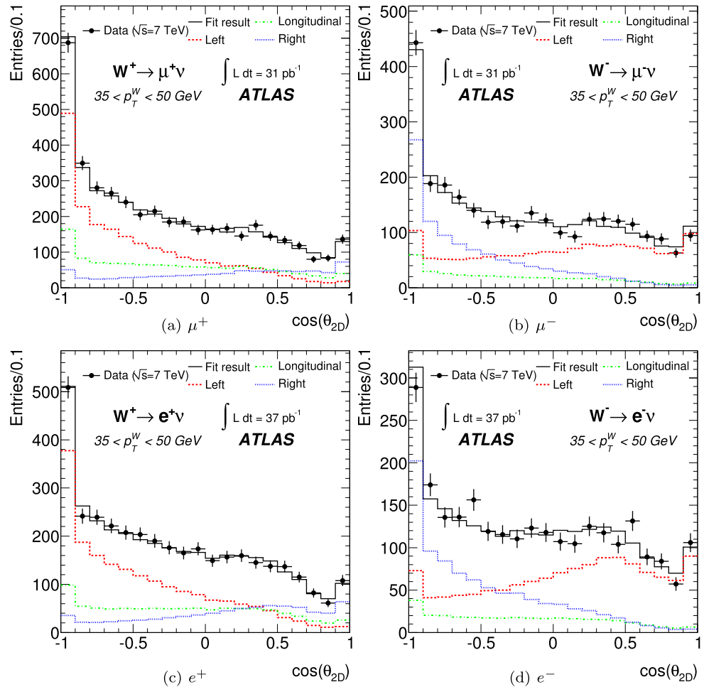
Fig. 7 Results of the fits to \cos\theta_{2D} distributions using helicity templates (built from MC@NLO), for W \rightarrow \mu\nu (top) and W \rightarrow e\nu (bottom) events in data with 35 < p_T^W < 50 GeV, after background subtraction. Each template distribution is represented: left-handed contribution (dashed line), longitudinal contribution (dotted-dashed line) and right-handed contribution (dotted line)
