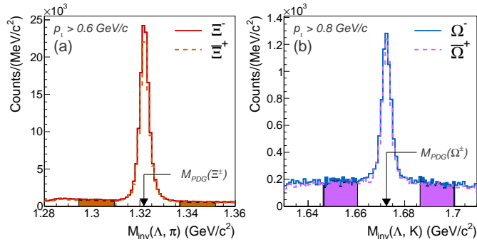
Fig. 1: The invariant mass distributions of \Xi^- (a) and \Omega^- (b) baryon candidates (solid histograms) and their antiparticles (dashed histograms). Also marked (in solid colour blocks) background sampling regions used in the signal extraction. The entire measured p_t range is presented.
