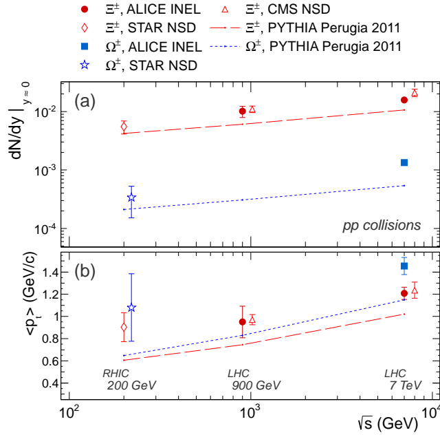
Fig. 3: (a) dN/dy and (b) \langle p_t \rangle of \Xi^\pm and \Omega^\pm as a function of collision energy. The STAR and CMS data are normalized to NSD (see text) events, STAR \Xi^\pm and \Omega^\pm are represented by open rhombuses and stars, respectively. CMS \Xi^\pm measurements are shown as open triangles, and ALICE \Xi^\pm and \Omega^\pm as filled circles and squares. Multi-strange baryons produced using PYTHIA Perugia 2011 simulation ( \Xi^\pm baryons as a long-dashed curve and \Omega^\pm baryons as a dashed curve) are plotted for reference. The uncertainties are added in quadrature.
