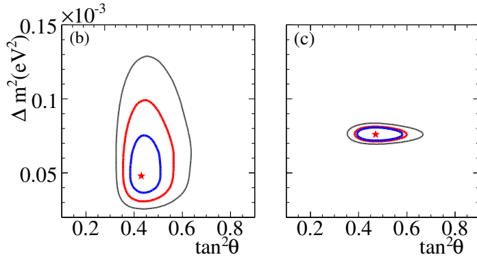
Fig. 34: Allowed regions (68%, 95% and 99.73% C.L.) for 2\nu oscillations from the global solar ( \nu_e ) data analysis (left) and from the combination of solar and KamLAND ( \bar{\nu}_e ) data (right), assuming CPT symmetry [91].
