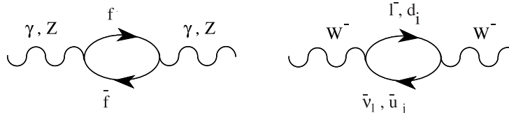
Fig. 18: Self-energy corrections to the gauge boson propagators.
