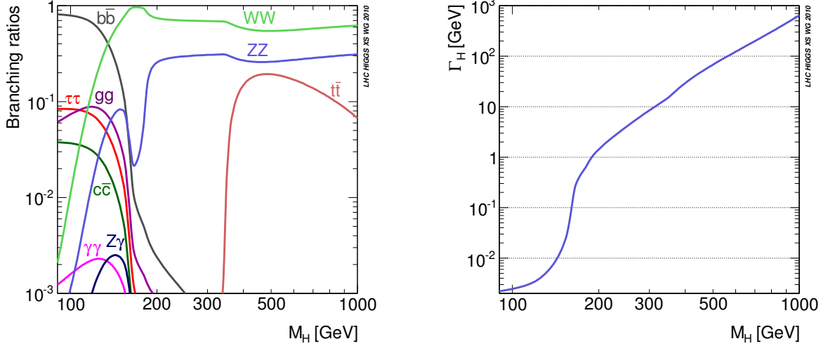
Fig. 28: Branching fractions of the different Higgs decay modes (left) and total decay width of the Higgs boson (right) as function of M_H [54].
