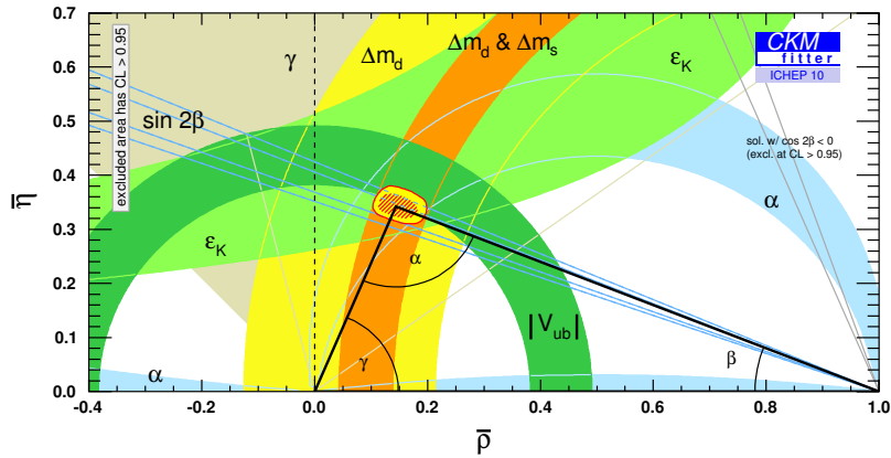
Fig. 31: Experimental constraints on the SM unitarity triangle [84].
