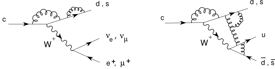
Fig. 30: Determinations of V_{ij} are done in semileptonic quark decays (left), where a single quark current is present. Hadronic decay modes (right) involve two different quark currents and are more affected by QCD effects (gluons can couple everywhere).
