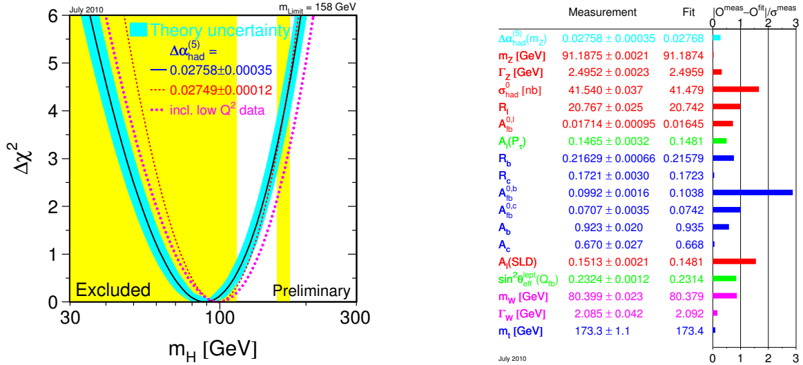
Fig. 24: \Delta\chi^2 versus M_H , from the global fit to the electroweak data. The vertical bands indicate the 95% exclusion limits from direct searches [34, 35].
