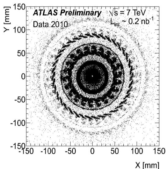
Figure 1: Example of a reconstruction of beam pipe and PIXEL position using nuclear interaction tomography [4].
