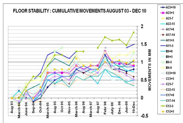
Figure 2: Time stability of the ATLAS cavern floor.
