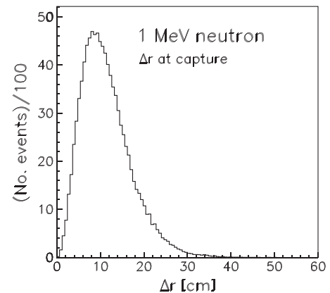
FIG. 8. Distribution of distances between the point of creation in the LSND scintillator medium of a 1 \text{ MeV} neutron and the point of capture on a free proton.
