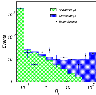
FIG. 2 (color online). “The R_\gamma distribution for events that satisfy the selection criteria for the primary \bar{\nu}_\mu \rightarrow \bar{\nu}_e oscillation search.” (Figure and its caption copied from Fig. 14 in Ref. [1]).
