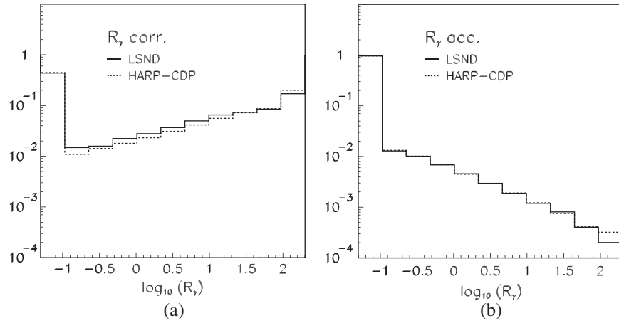
FIG. 12. The normalized LSND R_\gamma hypotheses (full lines) for correlated (left panel) and accidental (right panel) \gamma 's, compared with the respective normalized HARP-CDP R_\gamma hypotheses (broken lines); the former are a graphical representation (duly normalized) of the numbers listed in Table I; as for way the latter were obtained, see the text.
