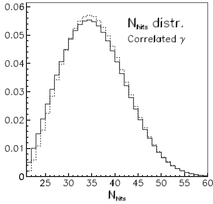
FIG. 11. Normalized distributions of the number of hit PMTs, N_{\text{hits}} , for correlated \gamma 's: as published by LSND (full line), and a variant (dotted line).
