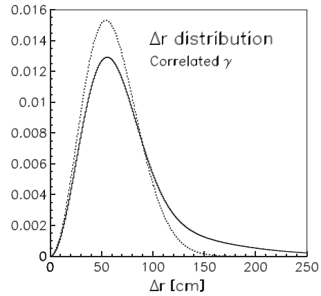
FIG. 9. Normalized distributions of the distance \Delta r for correlated \gamma ’s: as published by LSND (full line), and a variant (dotted line).
