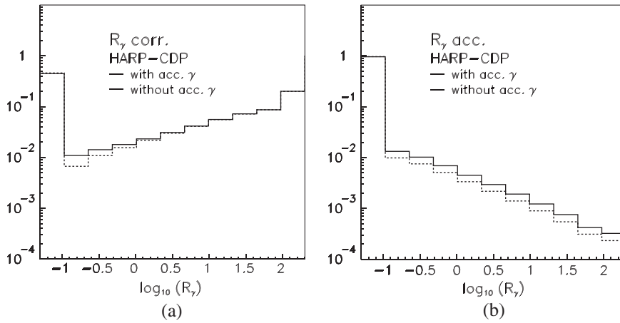
FIG. 13. The normalized HARP-CDP R_\gamma hypotheses for correlated (left panel) and accidental (right panel) \gamma 's with accidental \gamma 's at an effective rate of 1 kHz added (full lines), and without (broken lines).
