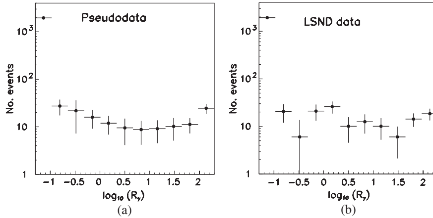
FIG. 15. Comparison of the “reference” R_\gamma distribution of the HARP-CDP pseudodata (left panel) with the R_\gamma distribution of the LSND data.
