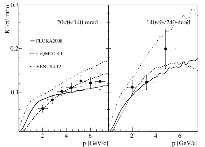
Figure 10: Ratio of K^+ to \pi^+ production cross sections in p+C interactions at 31 GeV/c. The ratios are presented as a function of laboratory momentum, p , in two intervals of polar angle \theta . Errors are calculated taking into account only statistical uncertainties. Predictions of hadron production models are superimposed.
