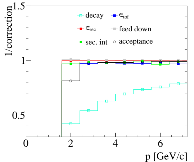
Figure 7: (Color online) Monte Carlo correction factors as a function of momentum calculated for the angular interval 20 < \theta < 140 mrad.
