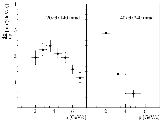
Figure 9: Differential cross sections for K^+ production in p+C interactions at 31 GeV/c. The spectra are presented as a function of laboratory momentum, p , in two intervals of polar angle, \theta . Error bars indicate statistical and systematic uncertainties added in quadrature. The overall uncertainty (2.5%) due to the normalization procedure is not included.
