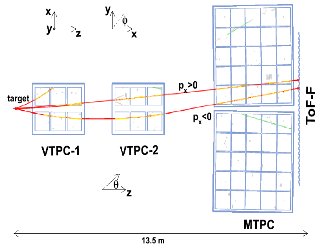
Figure 2: (Color online) Schematic drawing of the experimental apparatus (Sec. II) and a reconstructed p+C interaction event. Yellow (green) points indicate TPC clusters (not) associated to reconstructed primary tracks. Stars correspond to hits reconstructed in the ToF-F. Red lines are the fitted particle trajectories.
