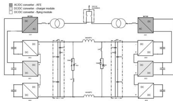
Figure 1: Topology of the power system.
