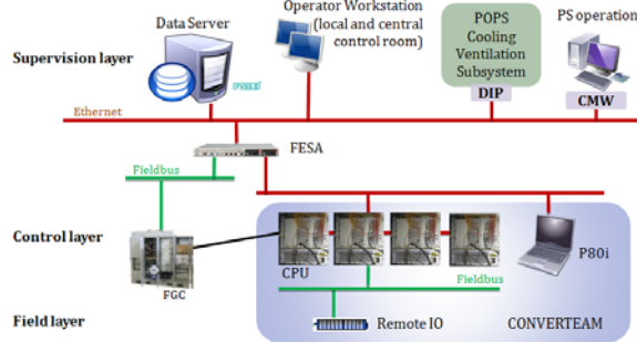
Figure 2: POPS control hardware architecture.
