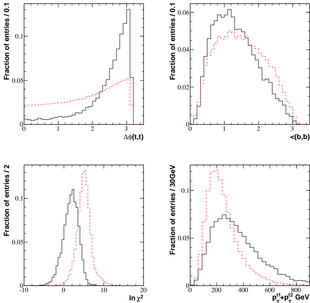
Figure 6.29: Histograms showing potential likelihood variables for correct (black/solid) and incorrect (red/dashed) jet combinations. All distributions are normalised to unit area.
