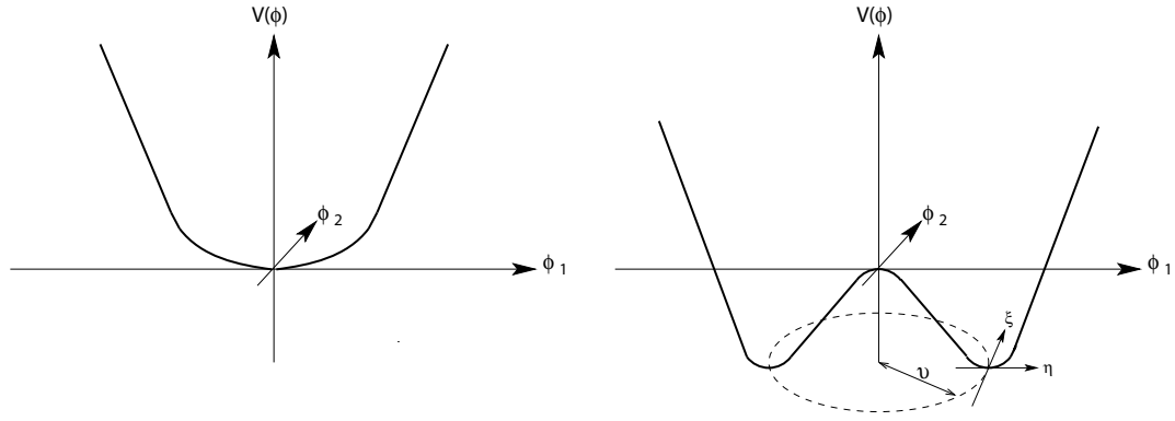
Figure 2.1: The potential V(\phi) for a complex scalar field for the case where \lambda > 0 and (a) \mu^2 > 0 (b) \mu^2 < 0 .
