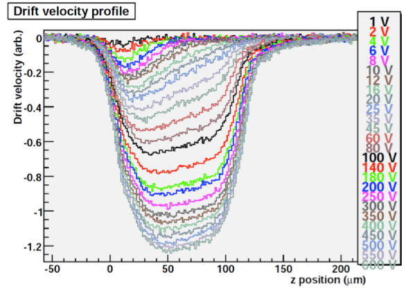
Figure 6: Drift velocity profile (el. Field) obtained with Edge-TCT measurement on a 120\mu m BabySTD Stripsensor. Here z is the coordinate perpendicular to the sensor plane
