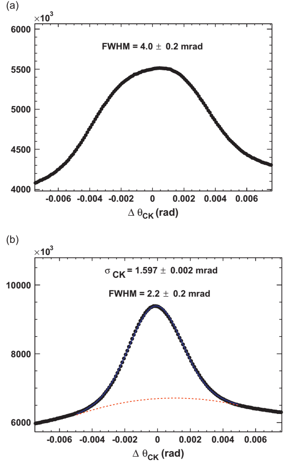
Fig. 15. The per-photon Cherenkov angle resolution in 2011 collision data: (a) before MDCS distortion correction applied and (b) after MDCS distortion correction applied.
