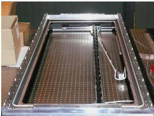
Fig. 6. A photograph of one MDCS system, installed in a photon funnel prior to installation in RICH1. The light bar is seen extended at \sim 1/3 of its full travel. During RICH operation, it is folded away into its parked position.
