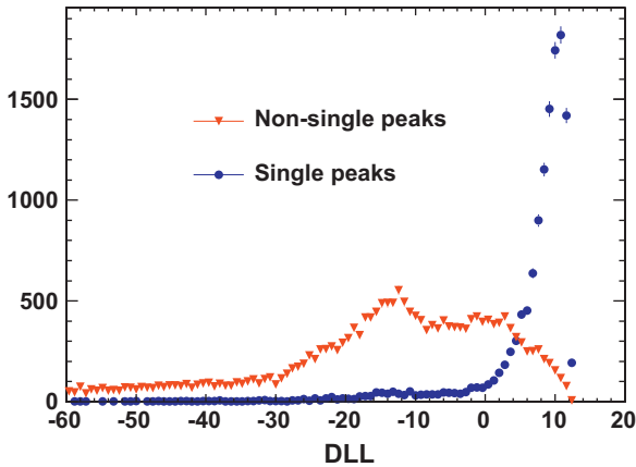
Fig. 10. DLL distribution of the peak fitting, showing single peaks (circles) and non-single peaks (triangles).
