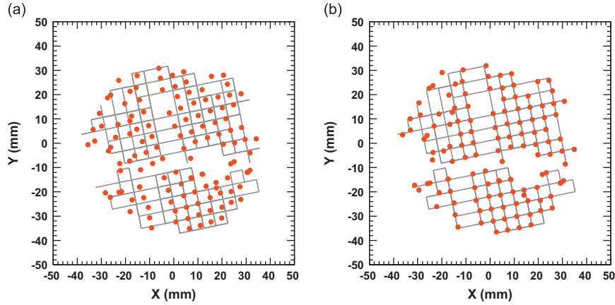
Fig. 11. MDSCS distortion correction applied to a typical HPD: (a) before distortion correction and (b) after distortion correction. The cleaned peak positions at the photocathode before and after correction are shown as dots. The expected grid patterns from two LED units are superimposed.
