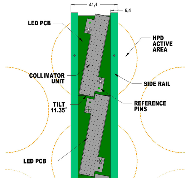
Fig. 4. A close-up of the light bar, showing two full LED PCB units, as viewed from the HPD array. The side rails are epoxied to the LED PCB, forming a U-channel in which the LED arrays plus collimator units are positioned. The LED array is covered by the collimator unit in this view. Dimensions are in mm.
