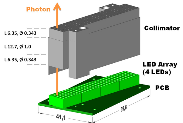
Fig. 5. An exploded view of a single LED PCB unit. Light is emitted from a given LED in the array into its collimator, encountering three segments of different lengths and diameters (as indicated). If not absorbed, the light emerges upwards toward the HPD array, which has its entrance window facing down at 85 mm distance (not shown). Dimensions are in mm.
