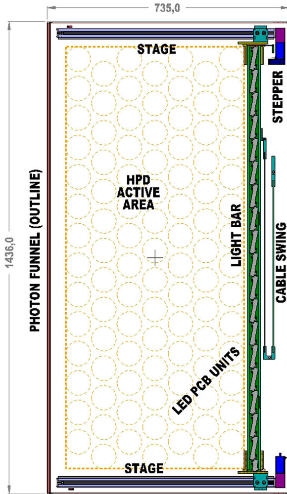
Fig. 3. MDCS overall system drawing. In this view, HPDs are located above the system, facing down (into page). Their projected positions are denoted by dotted circles. The light bar movement is horizontal, stepping incrementally in front of the HPDs, with a changing LED pattern at each step; it is shown here in its fully retracted (parked) position. The entire system fits within the photon funnel.
