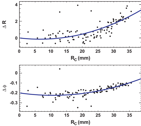
Fig. 12. Polynomial fits of distortion pairs \Delta R and \Delta\phi as a function of R_C .
