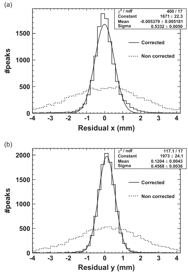
Fig. 13. Typical position resolution of corrected peak positions in calibration data, as measured at the HPD quartz window, for (a) x (LHCb pixel) direction, and (b) y (ALICE pixel) direction. The uncorrected peak positions are indicated by the dashed histogram.
