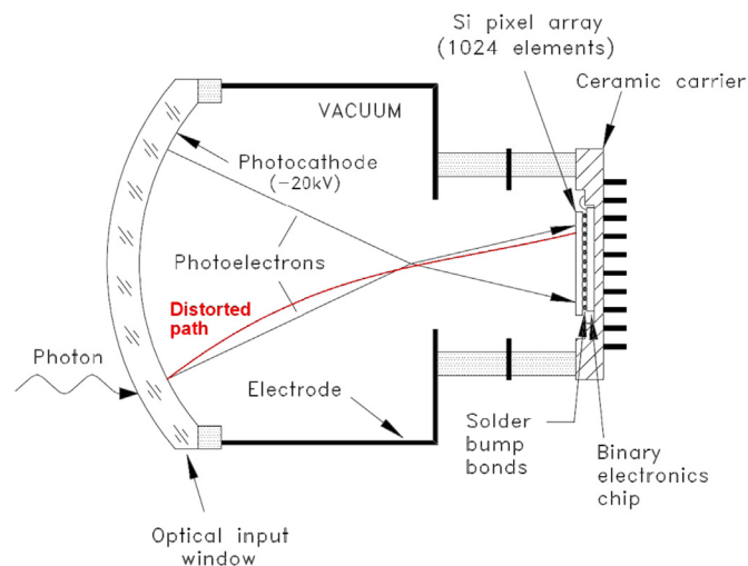
Fig. 2. Schematic view of the LHCb RICH HPD. Photons impinge on the spherical quartz input window and are converted to photoelectrons which are cross-focused onto a silicon pixel array with custom readout. A typical photoelectron trajectory that is distorted due to an external magnetic field is indicated.
