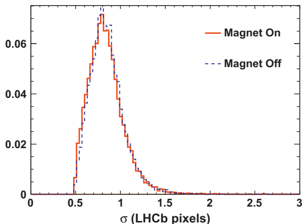
Fig. 8. The radial width \sigma of cleaned peaks, for magnet on data (solid) and magnet off data (dashed).
