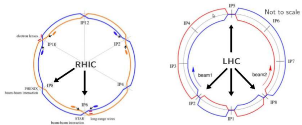
Figure 1: Schematic of RHIC and LHC rings with interaction points.
