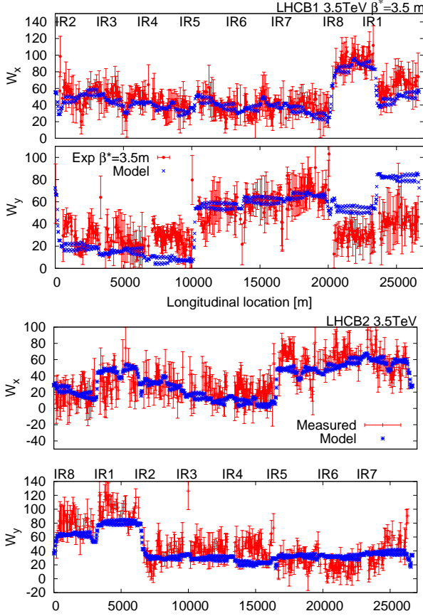
Figure 2: Chromatic W -functions for beam 1 and beam 2 in the LHC for 3.5 TeV at \beta^* = 3.5 m
