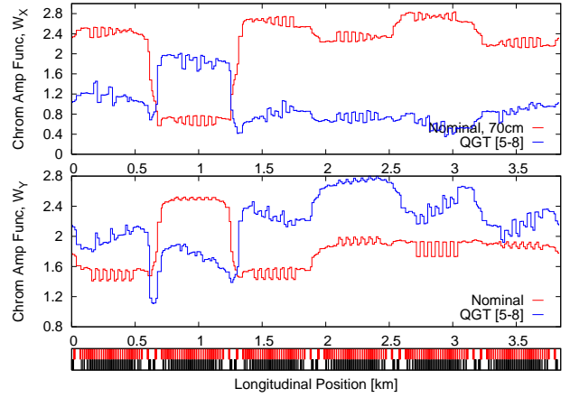
Figure 6: Chromatic W-functions for the nominal lattice at \beta^* = 0.7m and lattice with \gamma -T quadrupoles used to minimize them in the IR6 and IR8 regions.
