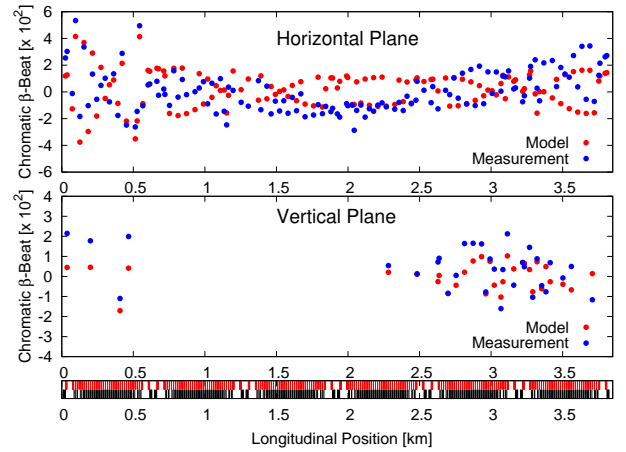
Figure 3: Chromatic \beta -beating in the Blue ring with gold ions at 100 GeV and 0.7m \beta^* .
