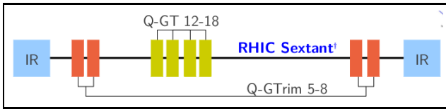
Figure 5: Schematic of the \gamma -T quadrupoles in one of the RHIC arc sections.
