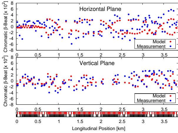
Figure 4: Chromatic \beta -beating in the Yellow ring with gold ions at 100 GeV and 0.7m \beta^* .
