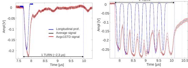
Figure 4: ACEM data for the TOF beam (left) and the CNGS beam (right). Red: BLM signal. Blue: WCM signal
