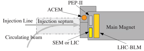
Figure 2: Sketch of BLMs installation in the PS injection
