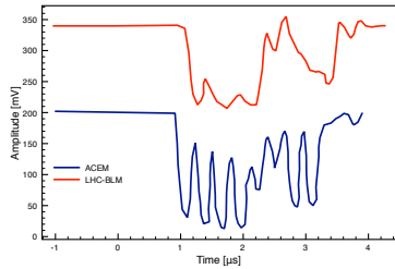
Figure 6: ACEM signal (blue) compared to the LHC-BLM (red) for the CNGS case. The vertical offset is introduced artificially to separate the two curves
