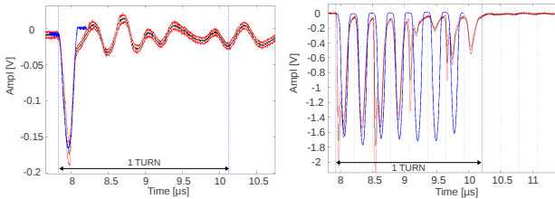
Figure 5: PEP-II data for the TOF beam (left) and the CNGS beam (right). Red: BLM signal. Blue: WCM signal
