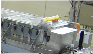
Figure 1: PS main magnet with a LHC-type BLM (yellow cylinder on top of the magnet) and an ACEM (orange cylinder in front of the magnet)
