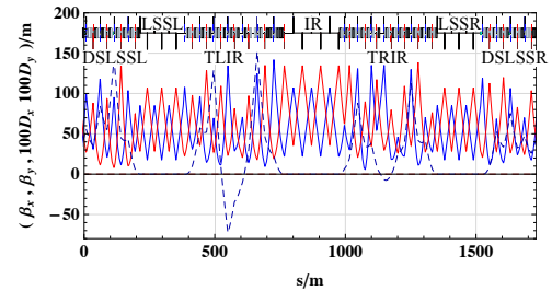
Figure 7: Bypass layout and optics in Point 1.
