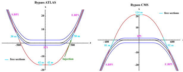
Figure 3: Final bypass design: The LHC p-ring is shown in black, the e-ring in red and the tunnel walls in blue. Dispersion free sections reserved for the installation of RF, wiggler(s), injection and other equipment are marked in light blue. The injection is marked in green in the right arc of the bypass in Point 1. Beginning and end of the bypass are marked as S.BP and E.BP.
