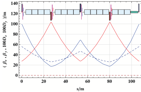
Figure 5: e-ring arc cell optics. One arc period consists of two asymmetric FODO cells. The horiz./vert. \beta -functions are shown in blue/red and the dispersion in dashed blue/red.
