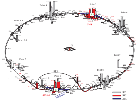
Figure 2: Schematic Layout of the LHeC: In grey the LEP tunnel now used for the LHC, in red the LHC extensions. The two LHeC bypasses are shown in blue. The RF is installed in the central straight section of the two bypasses. The bypass around Point 1 also hosts the injection.
