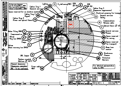
Figure 1: Cross-section of the LHC tunnel with the original space holder for the e-ring directly above the LHC cryostat and the shifted location (red) required to keep the overall circumference of e- and p-ring identical.
