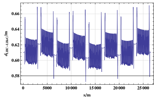
Figure 4: Radial distance between the p- and e-ring without bypasses.
