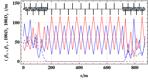
Figure 6: Insertion layout and optics at even points.
