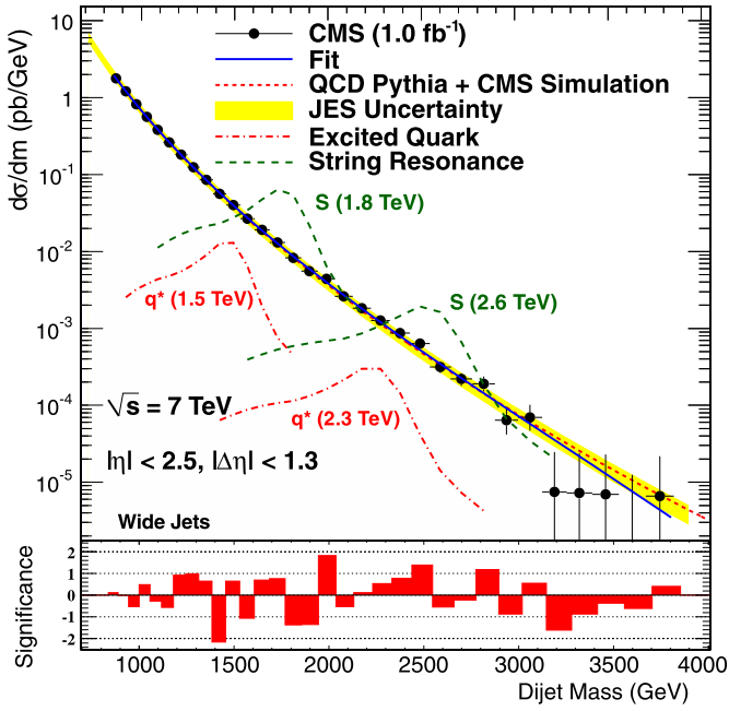
Fig. 2. Dijet mass spectrum from wide jets (points) compared to a smooth fit (solid) and to predictions [20] including detector simulation of QCD (short-dashed), excited quark signals (dot-dashed), and string resonance signals (long-dashed). The QCD prediction has been normalized to the data (see text). The error bars are statistical only. The shaded band shows the systematic uncertainty in the jet energy scale (JES). The bin-by-bin significance of the data-fit difference (see text) is shown at bottom.
