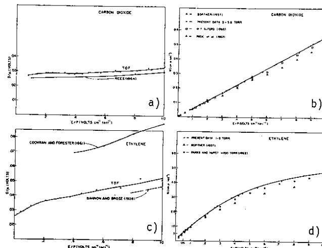
Fig. 7. Drift velocities and diffusion coefficients for \text{CO}_2 and \text{C}_2\text{H}_4 .
