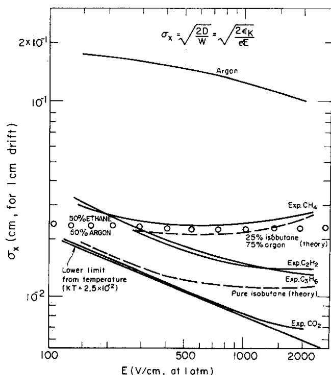
Fig. 3. Transverse diffusion \sigma_x after 1 cm of drift for various gases.
