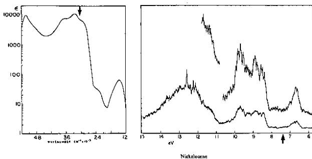
Fig. 14. a) Absorption spectrum of Nickelocene (in solution) around 337 nm. b) Photoionization spectrum of Nickelocene (from Ref. 31).
