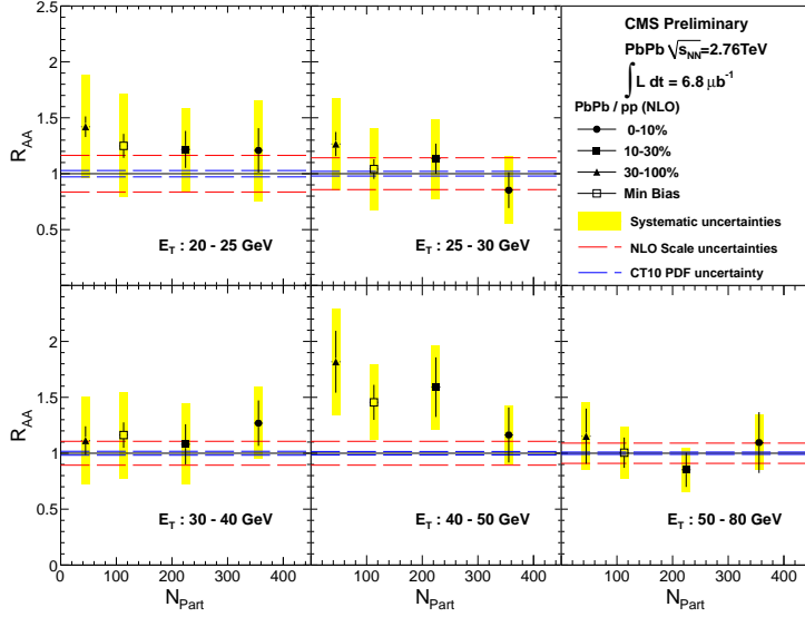
Figure 2: Nuclear modification factor R_{AA} as a function of N_{\text{part}} for the five different photon transverse energy intervals [3].
