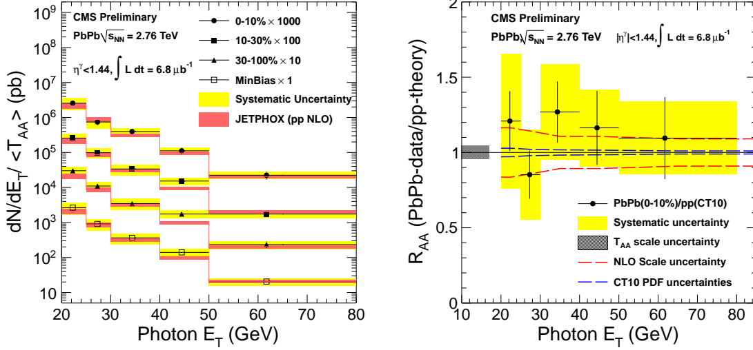
Figure 1: (Left Panel) Normalized isolated photon yields ( dN^\gamma/dE_T )/ T_{AA} in each centrality intervals and MinBias events [3]. (Right Panel) Nuclear modification factor R_{AA} as a function of the photon E_T measured in 0-10% central PbPb collisions over the T_{AA} -scaled pp JETPHOX prediction at \sqrt{s_{NN}} = 2.76 \text{ TeV} . The dashed lines are uncertainties from CT10 PDF [8] and NLO scale.
