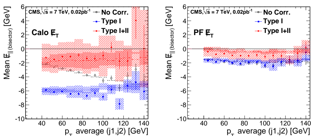
Figure 29. Mean values of \cancel{E}_{T||} as a function of average p_T of the two leading jets ( p_T^{\text{avg}} ) in dijet events compared with Monte Carlo simulation (dashed lines) for uncorrected, type-I corrected, and type-II corrected (left) Calo \cancel{E}_T and (right) PF \cancel{E}_T . The blue band on the distribution with type-I corrections reflects the uncertainty on the jet energy scale. The red band on the distribution with type-II corrections corresponds to the uncertainties on the jet energy scale and statistical uncertainties due to the size of the Z \rightarrow e^+e^- sample from which the correction for unclustered energies was derived.
