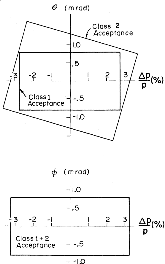
FIG. 6. The acceptance of the spectrometer for the two analyses performed on the data.
