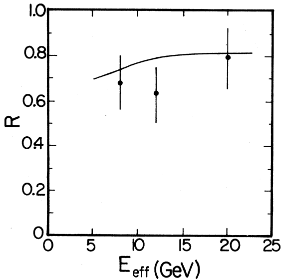
FIG. 23. The ratio R of \sigma_{\text{tot}}(K^*0p)/\sigma_{\text{tot}}(\bar{K}^*0p) as calculated from \pi^\pm p \rightarrow K^\pm X -inclusive scattering. The curve is the \sigma_{\text{tot}}(K^+p)/\sigma_{\text{tot}}(K^-p) ratio from data of Ref. 37.
