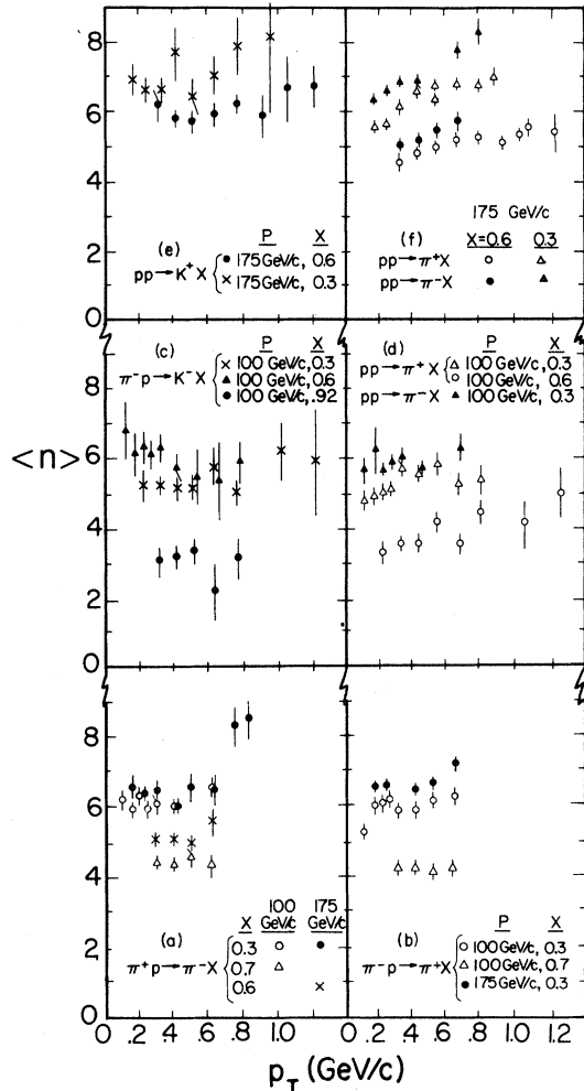
FIG. 27. Dependence of the associated-charged-particle multiplicity for particle-changing reactions a + p \rightarrow c + X on the transverse momentum of particle c at fixed x .
